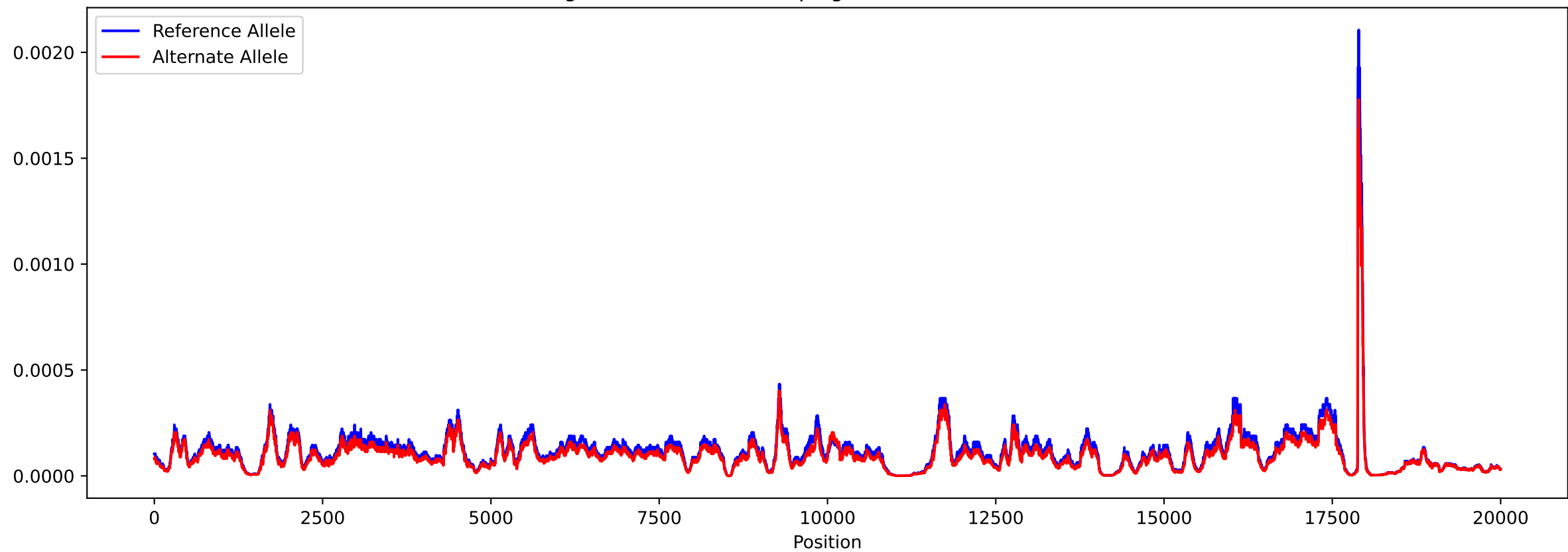
Predicted Negative Strand RNA-seq Signal for Reference vs Alternate Allele
