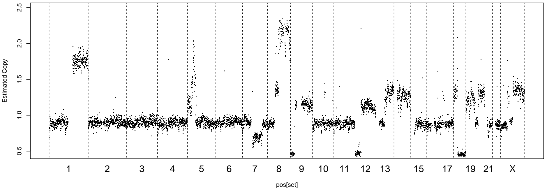
CG-corrected Readcount, MAD = 0.0829
