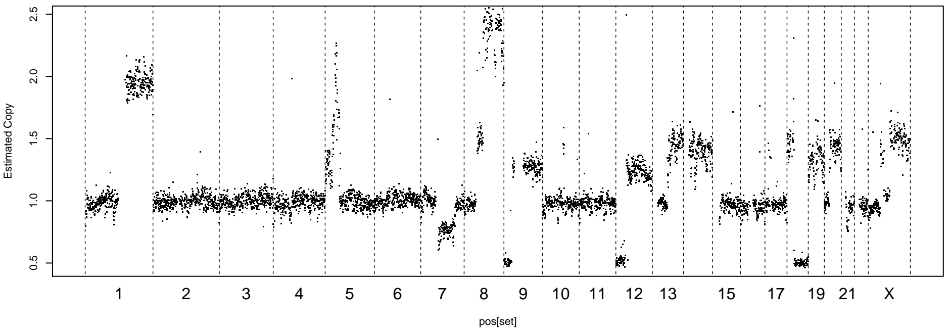
Mappability and GC-corrected Readcount, MAD = 0.0909
