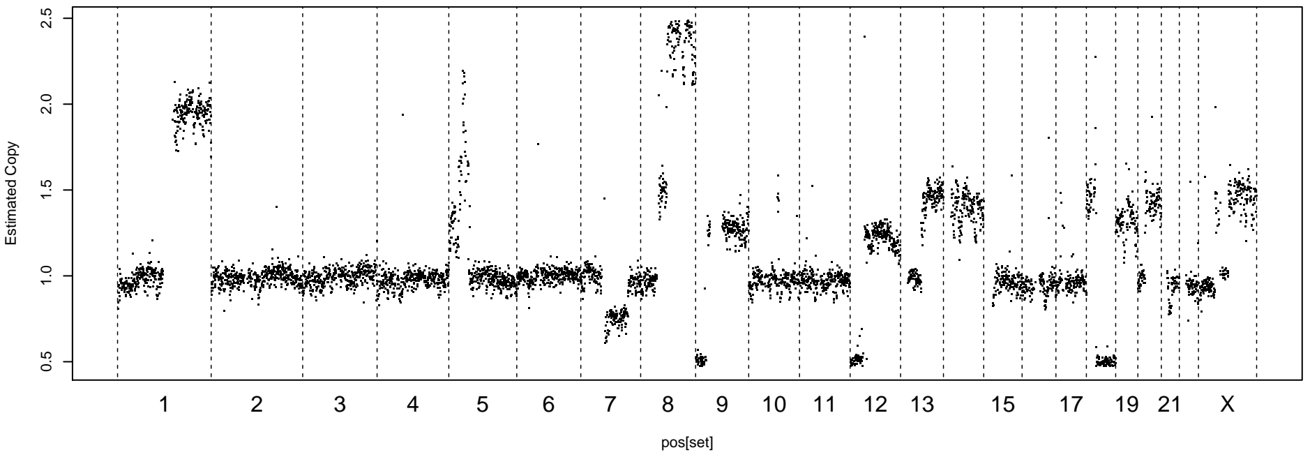
Uncorrected Readcount, MAD = 0.0854
