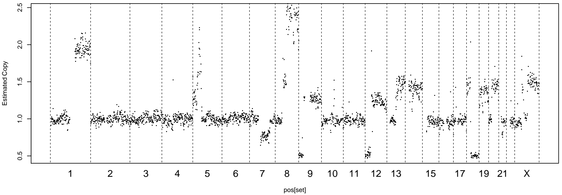
Mappability and GC-corrected Readcount, MAD = 0.0874
