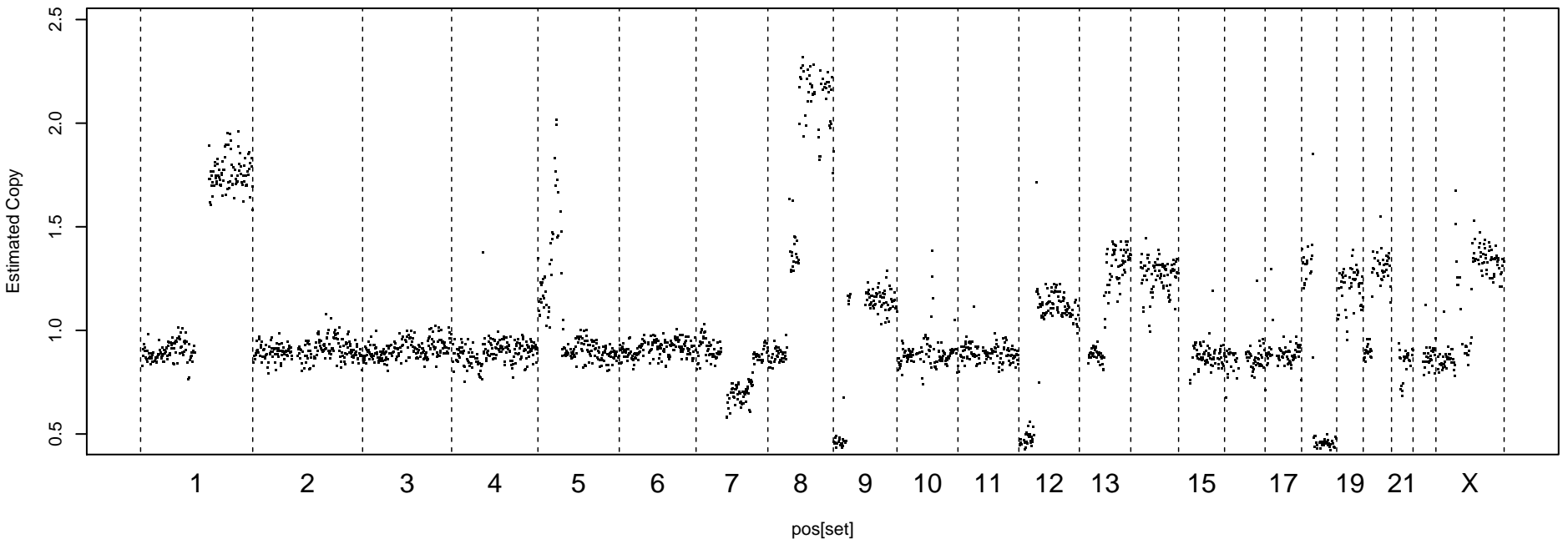
CG-corrected Readcount, MAD = 0.0792
