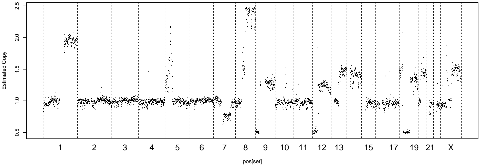
Uncorrected Readcount, MAD = 0.0734
