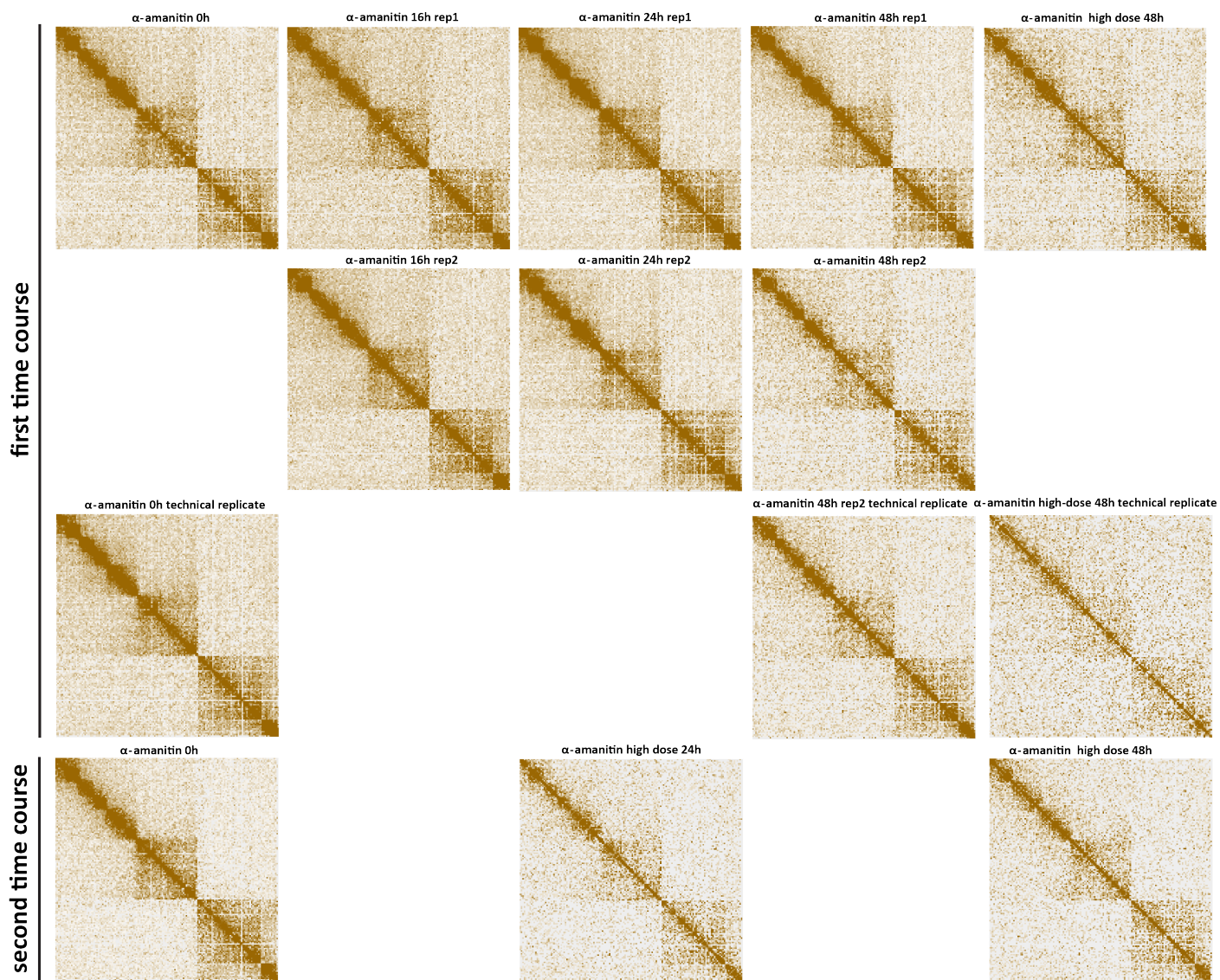
Supplementary Figure 24: Decompaction of dinoTADs upon transcriptional inhibition using \alpha -amanitin. Shown is pseudochromosome 18. Two time courses were carried out following the outline presented in Figure 2B.
