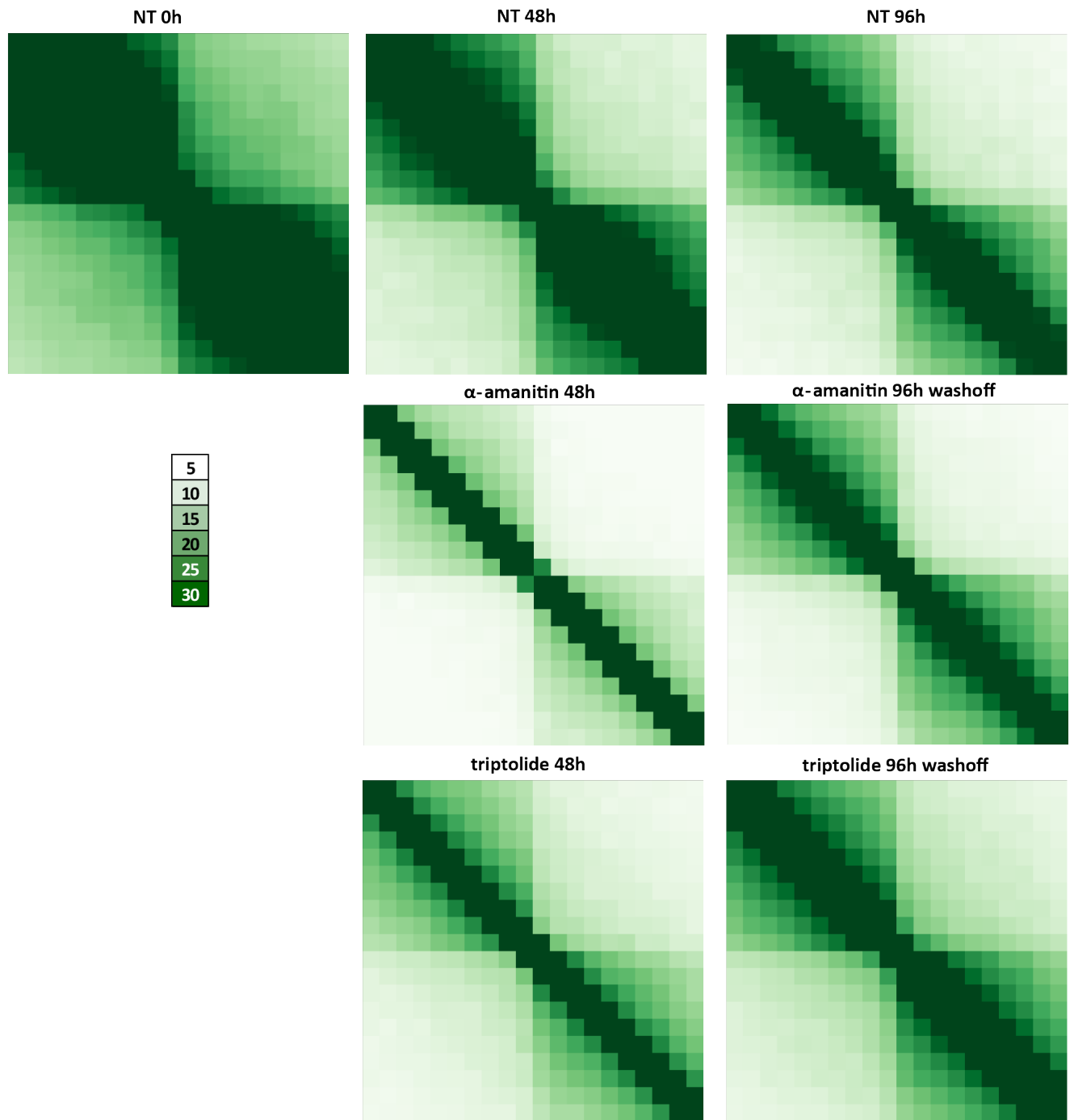
Supplementary Figure 33: Partial restoration of dinoTADs within 48 hours after removal of transcriptional inhibitors. Cells were treated with \alpha -amanitin or triptolide (“high” doses) for 48 hours, then the inhibitors was washed away, and cells were harvested another 48 hours later (“96 hours washoff”). Shown is a metaplot across all dinoTAD boundaries.
