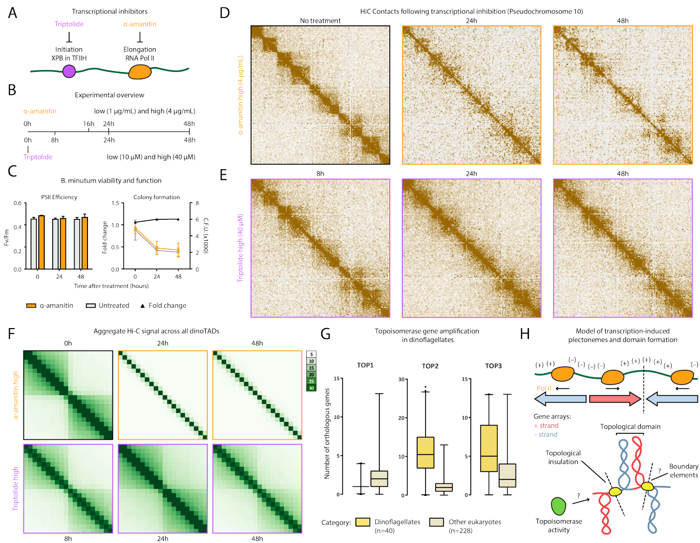
Figure 2: Decompanction of dinoTADs upon application of transcriptional inhibitors and the transcription-induced supercoiling model for their formation. Shown is pseudo-chromosome 10. (A-B) Outline of transcription inhibition time course experiments. (C) Comparison of cell function, measured by PSII photosynthetic efficiency, and cell viability, measured by colony formation (right), between \alpha -amanitin-treated and untreated cells. (D) KR-normalized Hi-C maps (50-kb resolution) show marked loss of dinoTADs after \alpha -amanitin treatment. (E) Hi-C maps show reduction of insulation at dinoTAD boundaries after triptolide treatment. (F) Metaplots of Hi-C signal around domain boundaries (50-kb resolution). (G) Amplification of TOP2 and TOP3 topoisomerases in dinoflagellates (based on MMETSP 7 transcriptome assemblies). (H) Transcription-induced supercoiling as driver of dinoflagellate chromatin folding. Transcribing polymerases introduce negative/positive DNA supercoiling behind/ahead of the transcription machinery. Interactions within supercoiled domains could explain the physical association of divergently-oriented arrays. Topological insulation could be driven by supercoiling-related effects, or by specific boundary elements.
