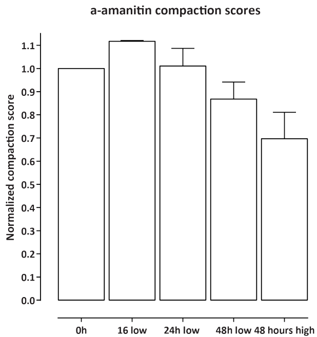
Response to Reviewers Figure 5: Quantifying dinoTAD compaction and decompaction using compaction scores. The compaction scores were calculated as the ratio of the average contacts within a dinoTAD at a distance of 250 kbp vs. the average contacts off-the diagonal (at 50,000 kb), then normalized to the matching untreated sample.
