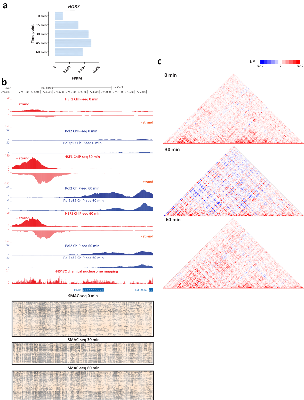
Supplementary Figure 65: Coordinated changes in chromatin accessibility and nucleosomal occupancy during the yeast stress response. Shown are changes in RNA Polymerase and HSF1 occupancy (measured by ChIP-seq), SMAC-seq profiles (1-bp resolution, 10-bp aggregate scores) and NMI profiles in the vicinity of the HOR7 gene.
