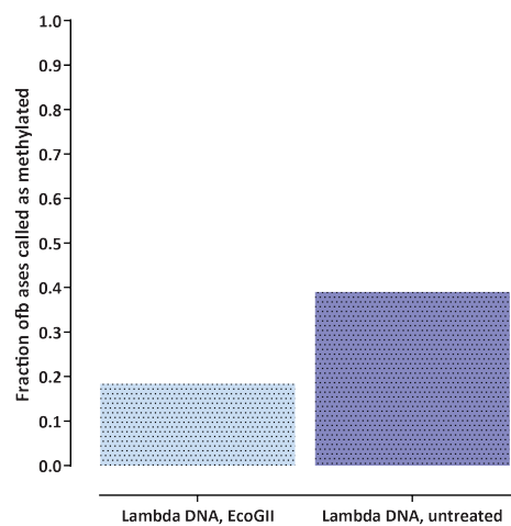
Supplementary Figure 6: Global m 6 A methylation levels in positive and negative controls (measured by nanopore sequencing). Unmethylated Lambda DNA was incubated with the EcoGII enzyme and then subjected to nanopore sequencing. Shown are the average methylation levels for A nucleotides. Note that completely methylated DNA molecules are not sequenced well on the nanopore platform, thus the methylation estimates in the treated sample are most likely underestimates.
