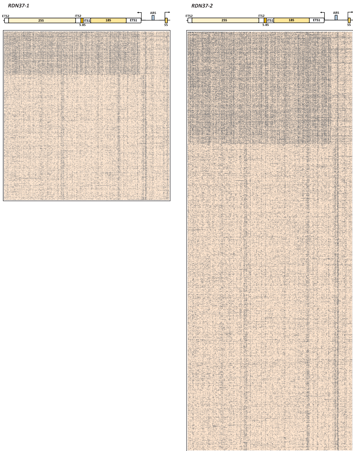
Supplementary Figure 40: SMAC-seq reveals the distribution of alternative chromatin states of rDNA arrays. Shown are all reads covering the RDN37-1 and RDN37-2 arrays in the RDN1 locus in the “diamide 30 min rep1” experiment (unfiltered reads, “aggregate” signal).
