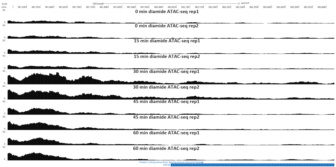
Supplementary Figure 78: Changes in chromatin accessibility during the yeast stress response around the HSP26 gene as measured by ATAC-seq.
