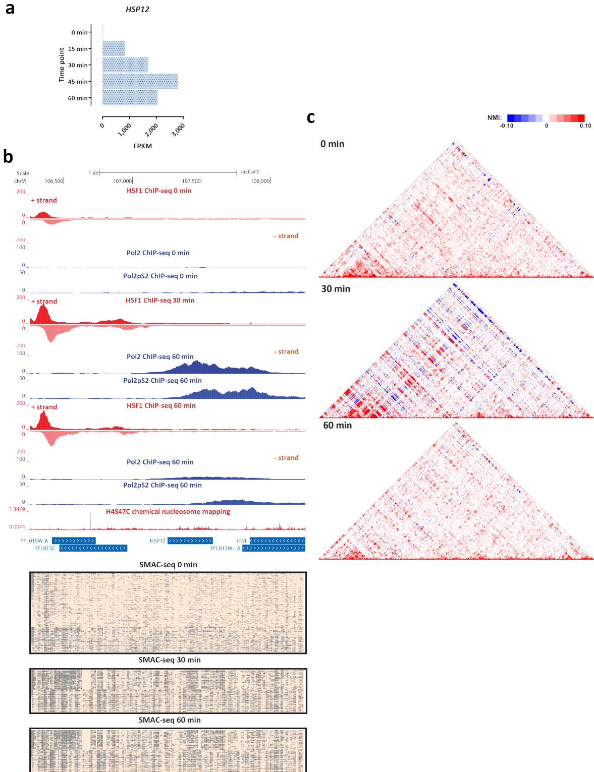
Supplementary Figure 67: Coordinated changes in chromatin accessibility and nucleosomal occupancy during the yeast stress response. Shown are changes in RNA Polymerase and HSF1 occupancy (measured by ChIP-seq), SMAC-seq profiles (1-bp resolution, 10-bp aggregate scores) and NMI profiles in the vicinity of the HSP12 gene.
