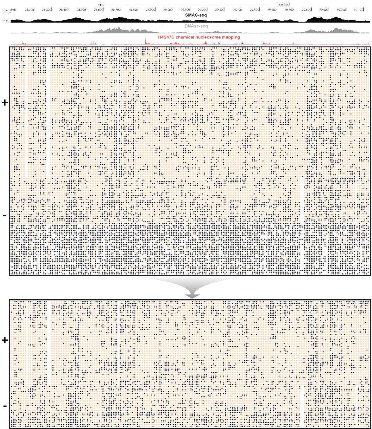
Supplementary Figure 30: Removal of potentially artifactual high-methylation reads. Shown is unfiltered SMAC-seq data and the same locus after removal of all reads containing a 1-kb \geq 75\% methylated stretch (average accessibility over 10 bp).
