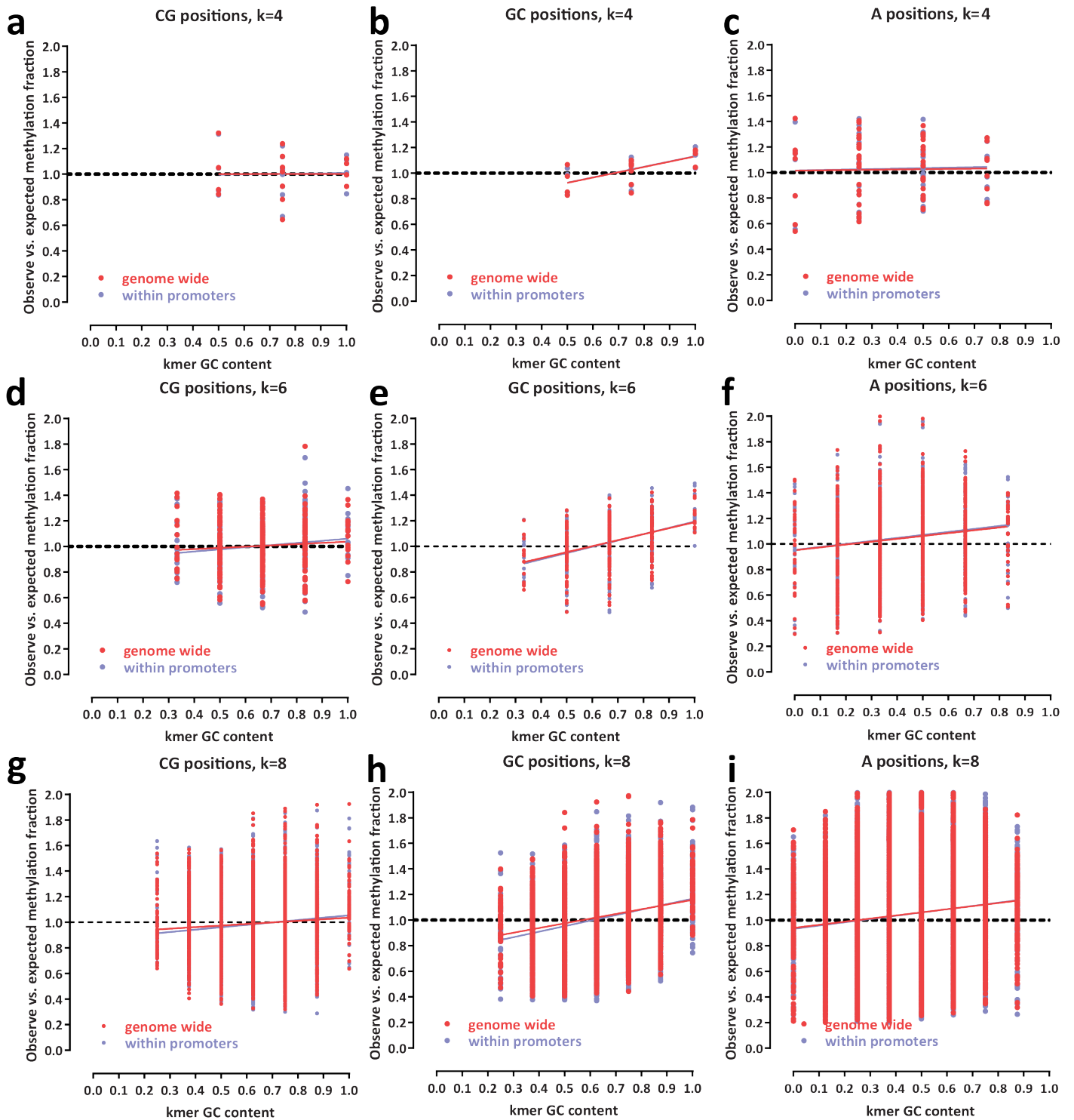
Supplementary Figure 20: Relationship between local GC content and enzymatic/methylated base calling bias. Shown is the ratio of observed versus expected fraction of methylated bases for each sequence context of size k , calculated as follows:
