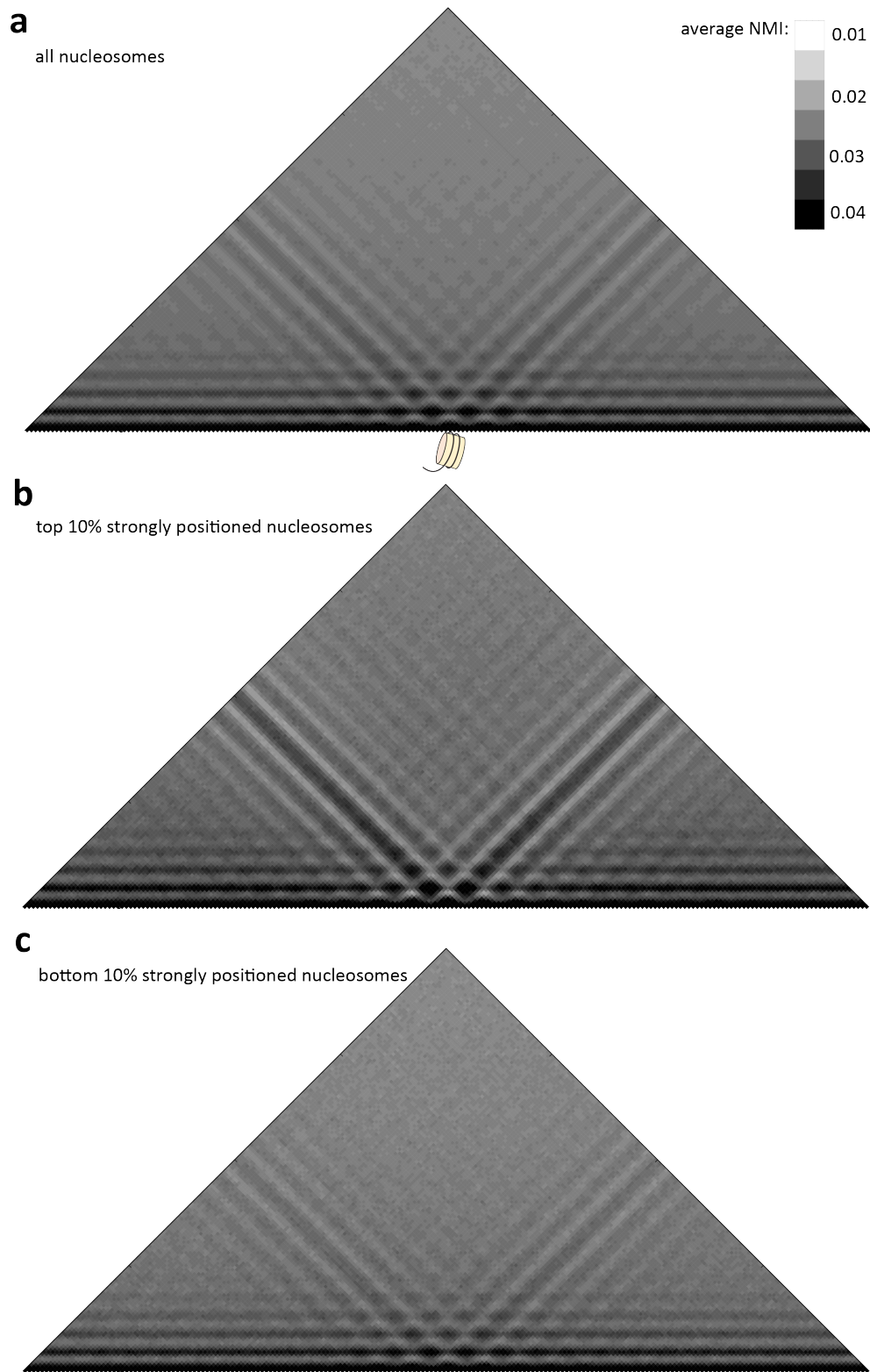
Supplementary Figure 56: Metanucleosome NMI profiles in the yeast genome. Shown are average NMI maps between all 20-bp segments centered on each positioned nucleosome in the genome (a), the top 10% strongly positioned nucleosomes (b), or the bottom 10% strongly positioned nucleosomes (c).
