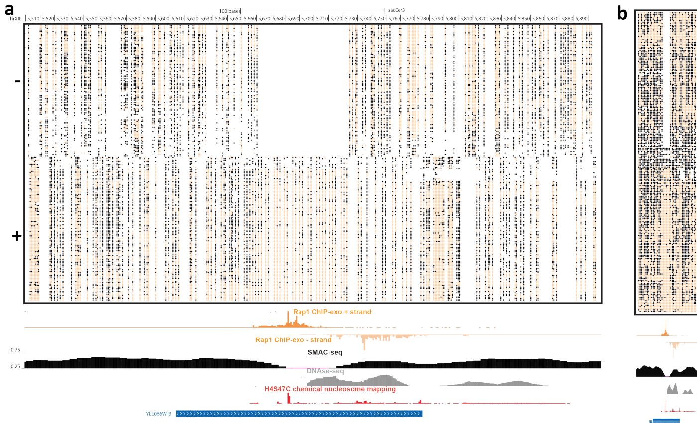
Supplementary Figure 52: Single-molecule footprinting associated with Rap1 occupancy. (a) Raw unfiltered nanopore reads fully spanning a 400-bp neighborhood of the subtelomeric region of chrXII, at single-bp resolution. White spaces indicate positions for which there is no data (i.e. no CG, GC or A). (b) Same as in (a), but at aggregated 10-bp resolution.
