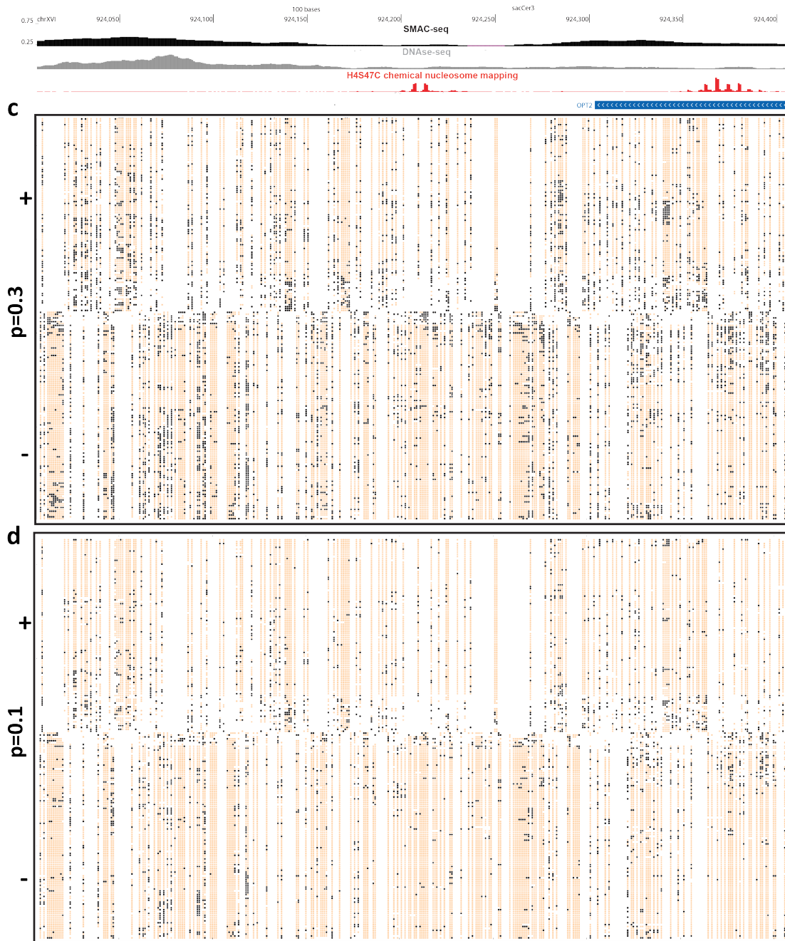
Supplementary Figure 16: Transformation of raw methylation probabilities into binary methylation calls. Shown is raw unfiltered SMAC-seq single-molecule data over a strongly positioned nucleosome on chrXVI (1-bp resolution). White spaces indicate positions for which there is no data (i.e. no CG, GC or A). (a) raw Tombo alternative model methylation probabilities; (b) p < 0.5 thresholding; (c) p < 0.3 thresholding; (d) p < 0.1 thresholding.
