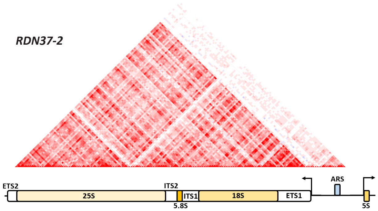
Supplementary Figure 43: NMI profile for the RDN37-2 array, as in Figure 3b.
