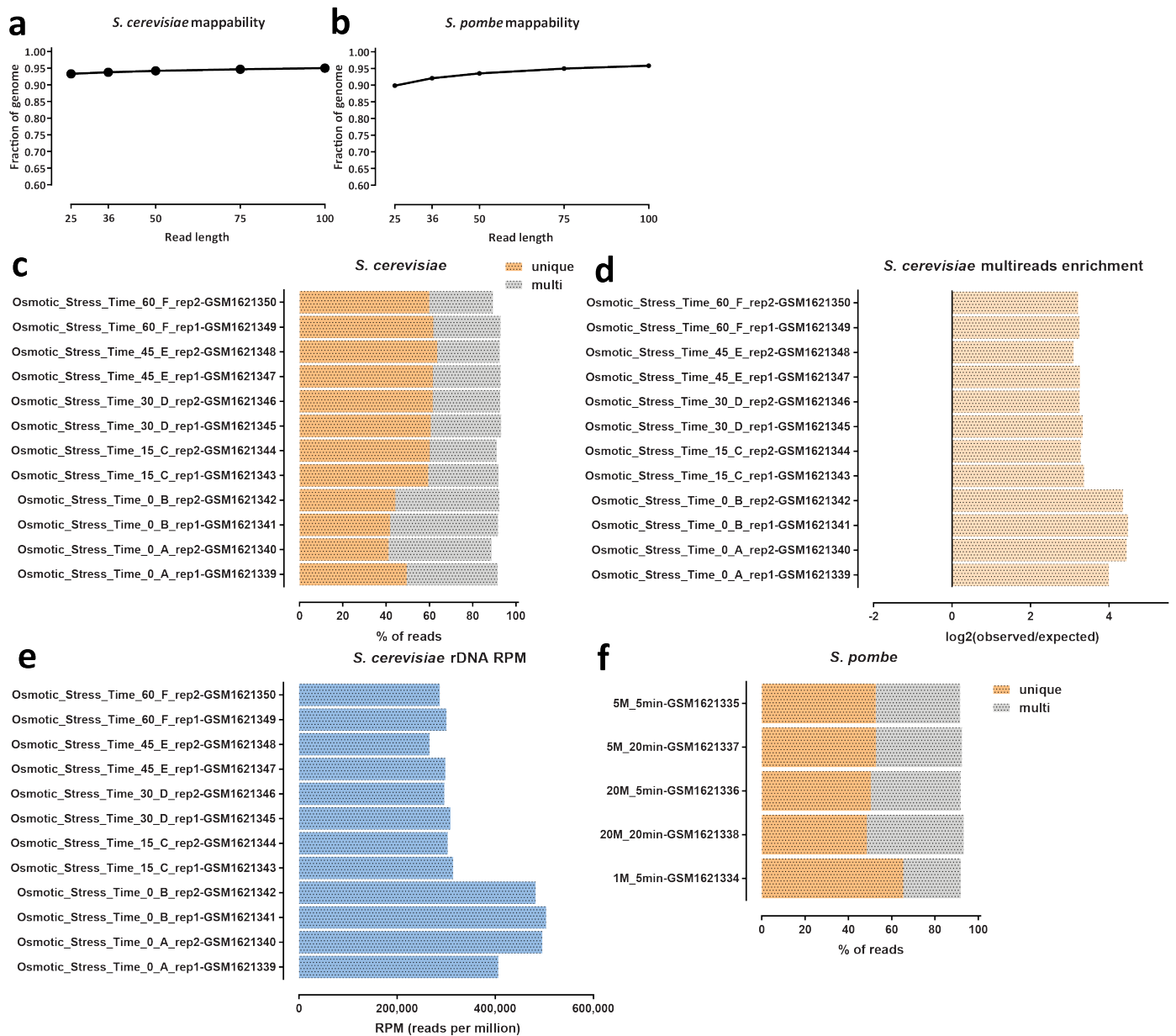
Supplementary Figure 39: Ribosomal DNA arrays are highly enriched for chromatin accessibility as measured by ATAC-seq. (a) Unique read mappability of the Saccharomyces cerevisiae genome as a function of read length (b) Unique read mappability of the Schizosaccharomyces pombe genome as a function of read length (c and d) Enrichment of multimapping reads in Saccharomyces cerevisiae ATAC-seq datasets (e) ATAC-seq multireads are highly enriched for rDNA-mapping reads (f) Enrichment of multimapping reads in Schizosaccharomyces pombe ATAC-seq datasets ATAC-seq datasets were obtained from Schep et al. 2015 53
