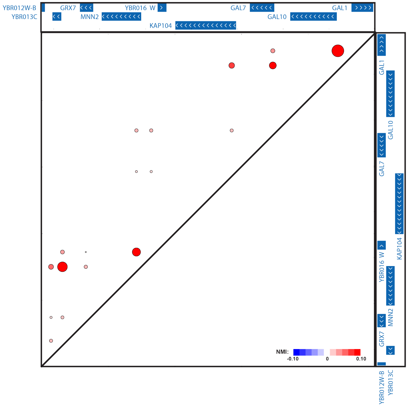
Supplementary Figure 59: Example of accessibility correlation between TSSs. Shown are accessibility correlations between all loci in the region with coordinates “chrII:265000-280000”. The size and color of the dots corresponds to their NMI scores.
