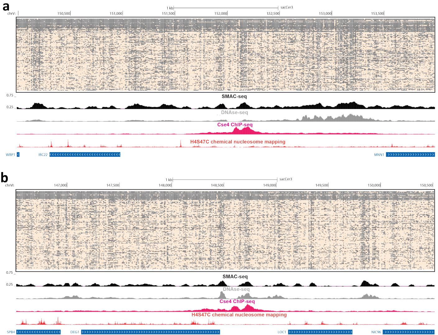
Supplementary Figure 33: Single-molecule long-read accessibility around well positioned centromeres. (a) Raw unfiltered nanopore reads fully spanning the 4-kilobase neighborhood of the centromere of S. cerevisiae chrV; (b) Raw unfiltered nanopore reads fully spanning the 4-kilobase neighborhood of the centromere of S. cerevisiae chrVI. In both cases, accessibility is shown at aggregated 10-bp resolution (see Methods section for details) for the single-molecule display, and aggregated over sliding (every 5 bases) 50-bp windows for the genome browser SMAC-seq track.
