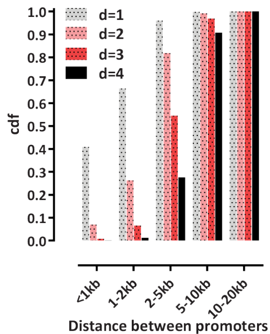
Supplementary Figure 2: Distance between regulatory elements (i.e. promoters in the case of S. cerevisiae ).
