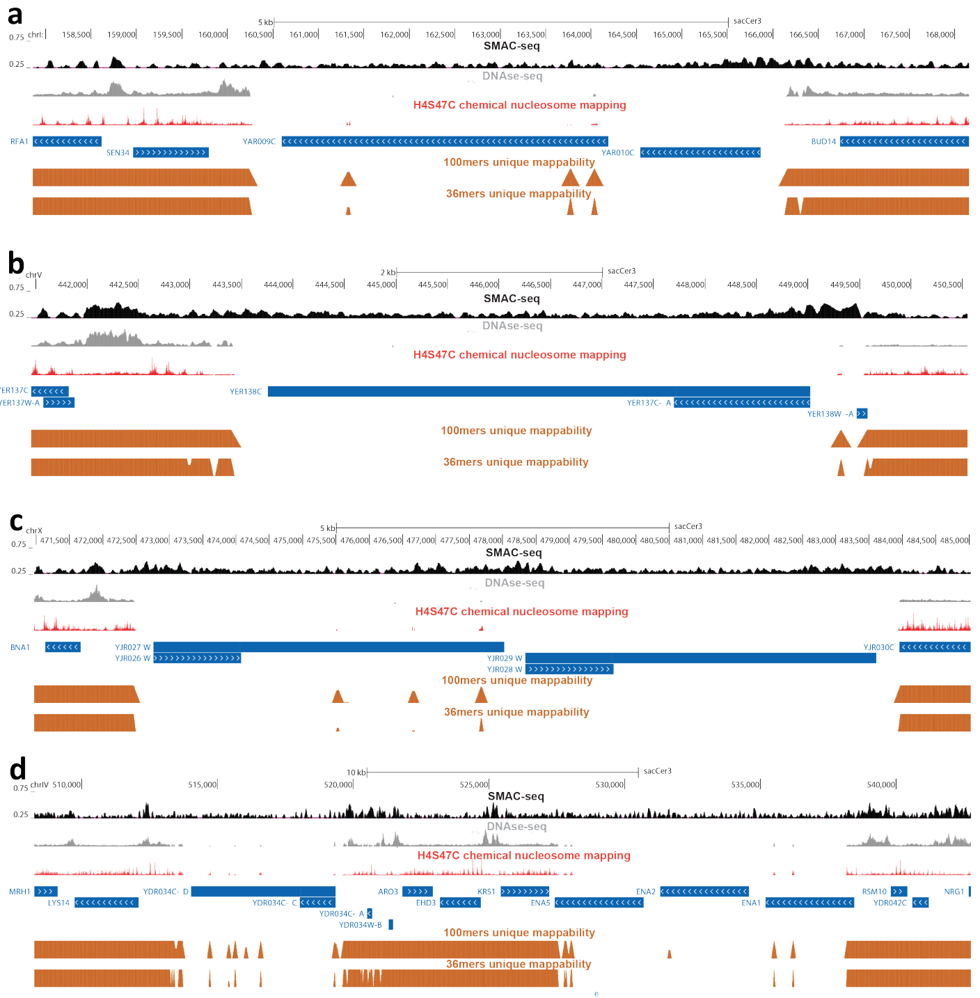
Supplementary Figure 27: SMAC-seq provides coverage of areas of the genome that cannot be uniquely mapped using short reads. Four different repetitive regions are shown (a, b, c and d) together with short read coverage for DNase-seq and chemical nucleosome mapping data and unique mappability tracks for 36mers and 100mers.
