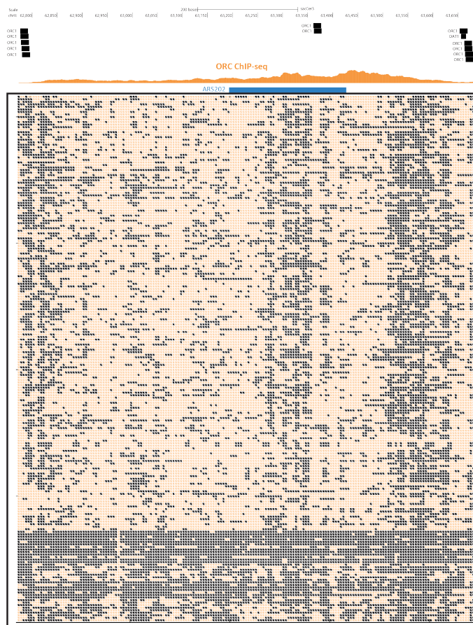
Supplementary Figure 52: Single-molecule footprinting associated with ORC occupancy. (a) Raw unfiltered nanopore reads fully spanning the neighborhood of an ARS site on chrII, at 5-bp aggregated resolution. White spaces indicate positions for which there is no data (i.e. no CG, GC or A).
