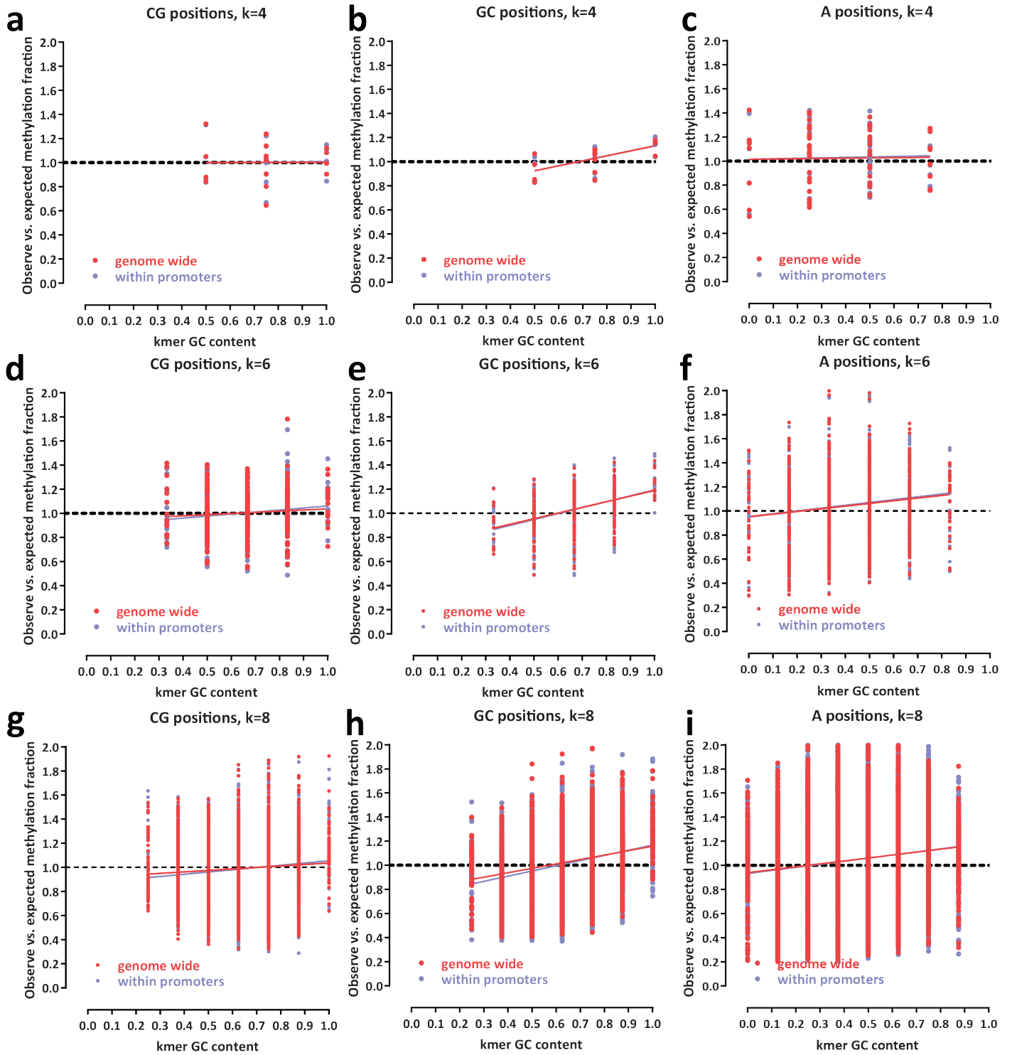
Supplementary Figure 19: Relationship between local GC content and enzymatic/methylated base calling bias. Shown is the ratio of observed versus expected fraction of methylated bases for each sequence context of size k , calculated as follows:
