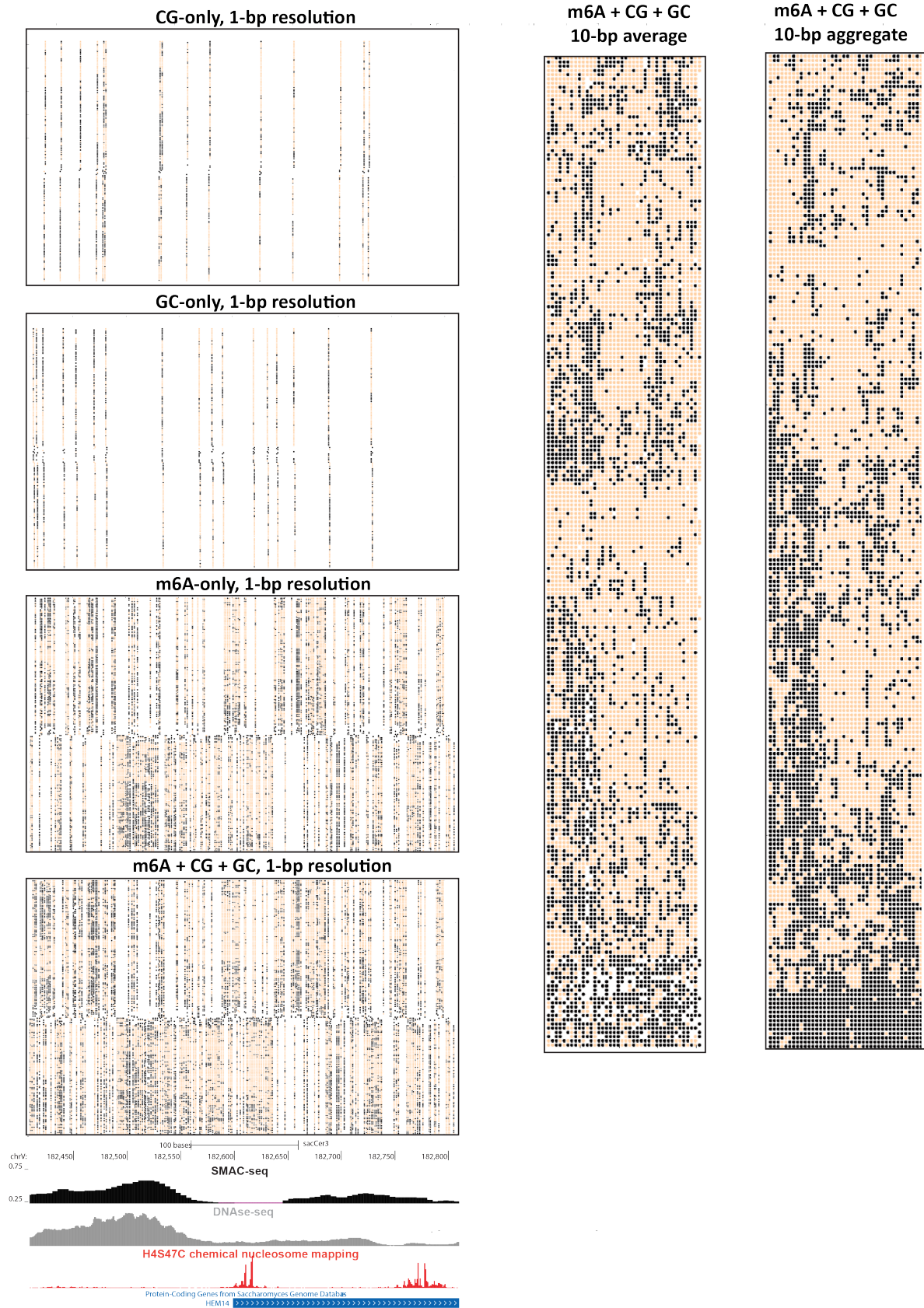
Supplementary Figure 7: Impact of the addition of m^6A on assay resolution. Shown is the raw unfiltered nanopore read coverage around a strongly positioned +1 nucleosome, considering only CG, only GC, only m^6A , and all bases at 1-bp resolution as well as all bases at averaged and aggregated 10-bp resolution. White spaces indicate positions for which there is no data (i.e. no CG, GC or A).
