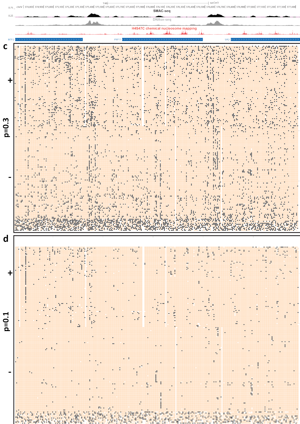
Supplementary Figure 16: Transformation of raw methylation probabilities into binary methylation calls. Shown is raw unfiltered SMAC-seq single-molecule data over a ~2.8kb locus on chrIV (10-bp average for all panels). White spaces indicate positions for which there is no data (i.e. no CG, GC or A). (a) raw Tombo alternative model methylation probabilities; (b) p < 0.5 thresholding; (d) p < 0.3 thresholding; (d) p < 0.1 thresholding.
