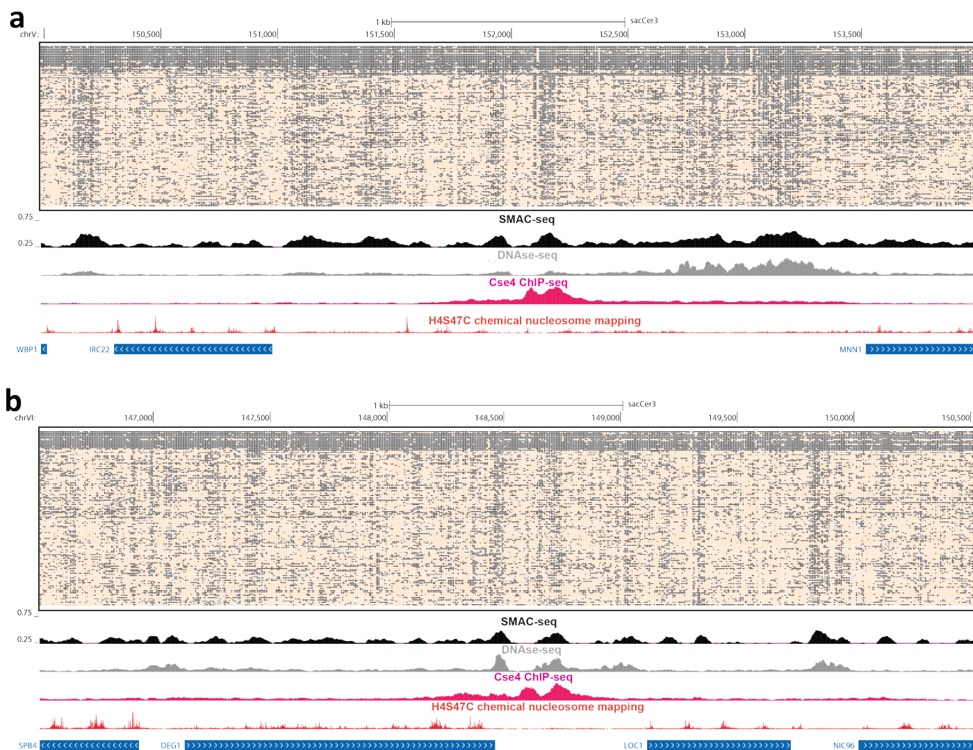
Supplementary Figure 32: Single-molecule long-read accessibility around well positioned centromeres. (a) Raw unfiltered nanopore reads fully spanning the 4-kilobase neighborhood of the centromere of S. cerevisiae chrV; (b) Raw unfiltered nanopore reads fully spanning the 4-kilobase neighborhood of the centromere of S. cerevisiae chrVI. In both cases, accessibility is shown at aggregated 10-bp resolution (see Methods section for details) for the single-molecule display, and aggregated over sliding (every 5 bases) 50-bp windows for the genome browser SMAC-seq track.
