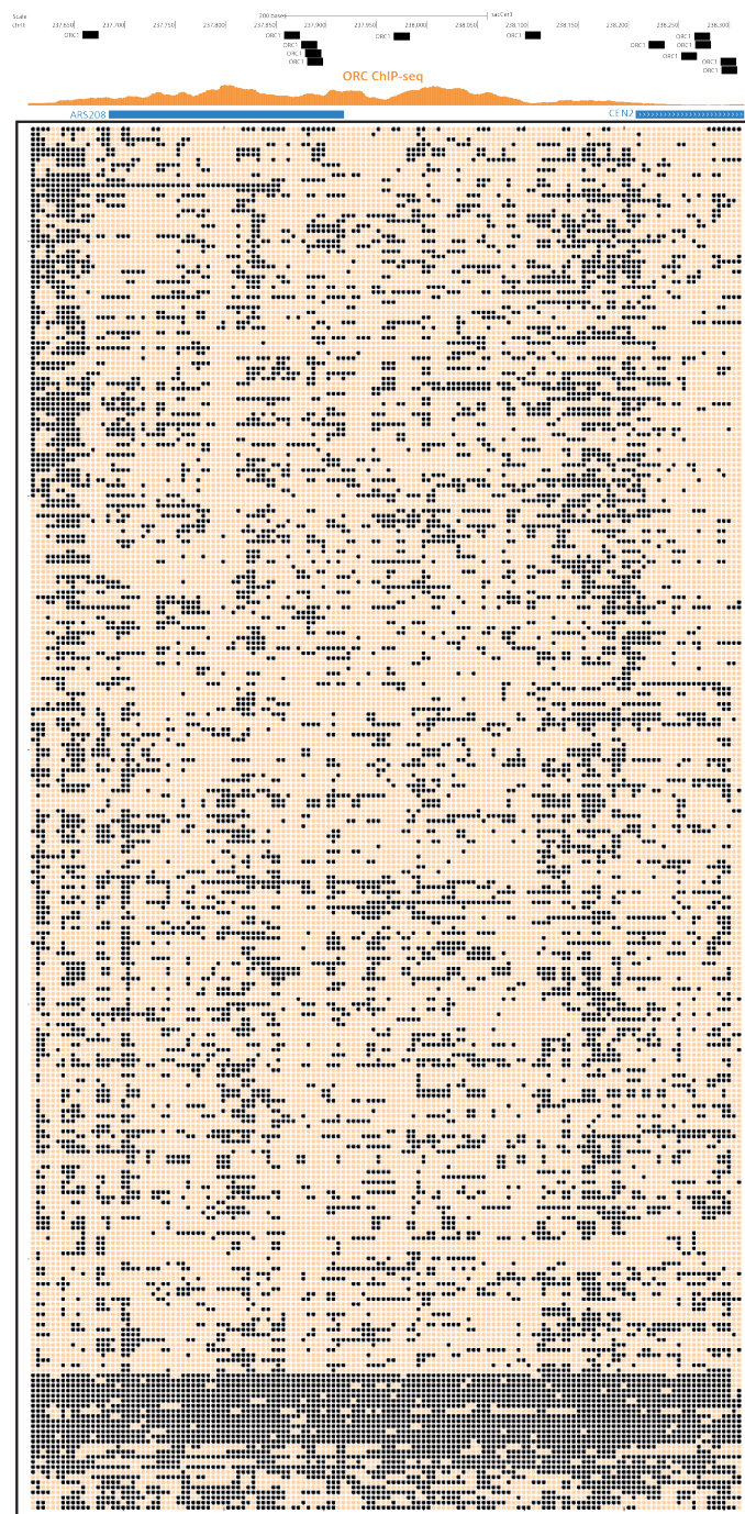
Supplementary Figure 54: Single-molecule footprinting associated with ORC occupancy. (a) Raw unfiltered nanopore reads fully spanning the neighborhood of an ARS site on chrII, at 5-bp aggregated resolution. White spaces indicate positions for which there is no data (i.e. no CG, GC or A).
