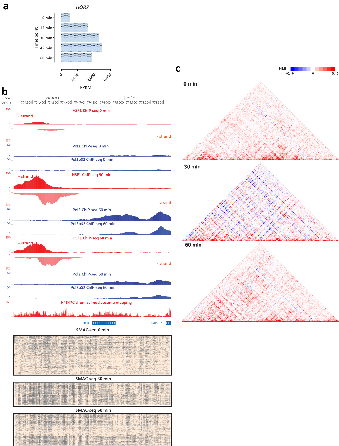
Supplementary Figure 64: Coordinated changes in chromatin accessibility and nucleosomal occupancy during the yeast stress response. Shown are changes in RNA Polymerase and HSF1 occupancy (measured by ChIP-seq), SMAC-seq profiles (1-bp resolution, 10-bp aggregate scores) and NMI profiles in the vicinity of the HOR7 gene.
