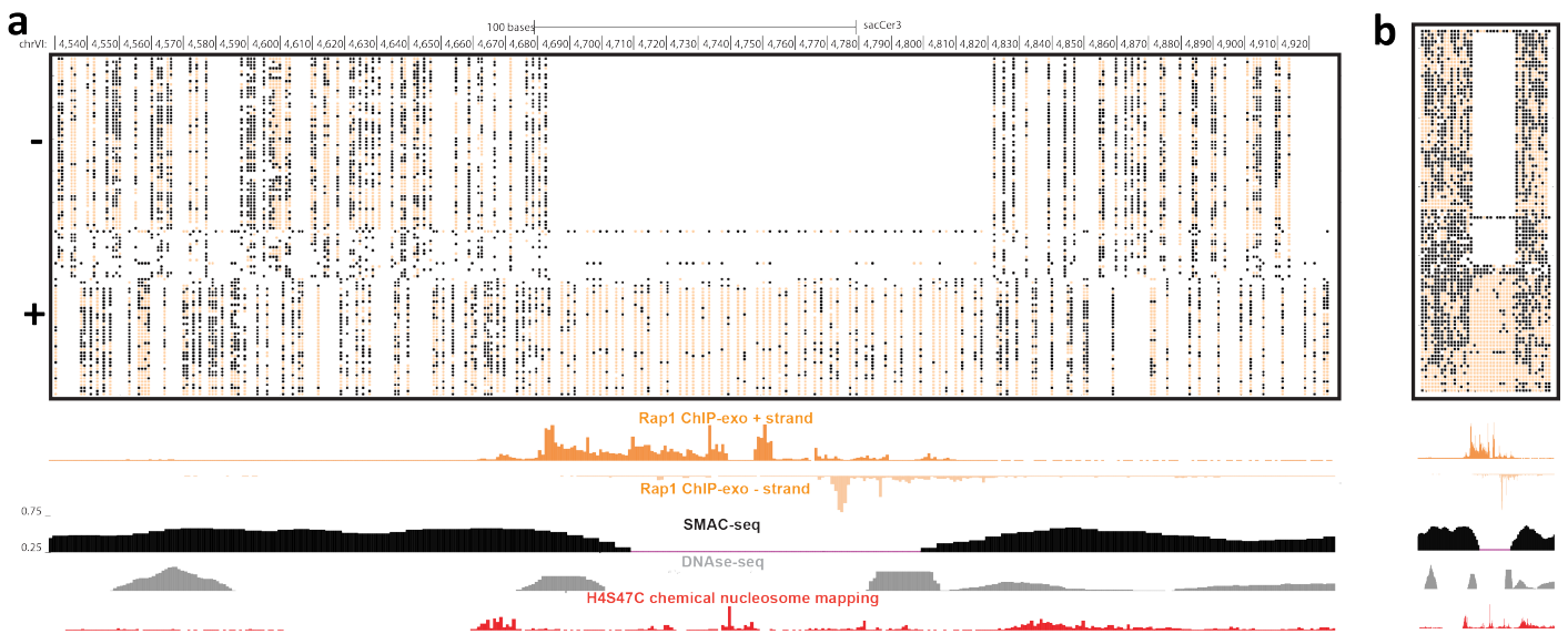
Supplementary Figure 50: Single-molecule footprinting associated with Rap1 occupancy. (a) Raw unfiltered nanopore reads fully spanning a 400-bp neighborhood of the subtelomeric region of chrVI, at single-bp resolution. White spaces indicate positions for which there is no data (i.e. no CG, GC or A). (b) Same as in (a), but at aggregated 10-bp resolution.
