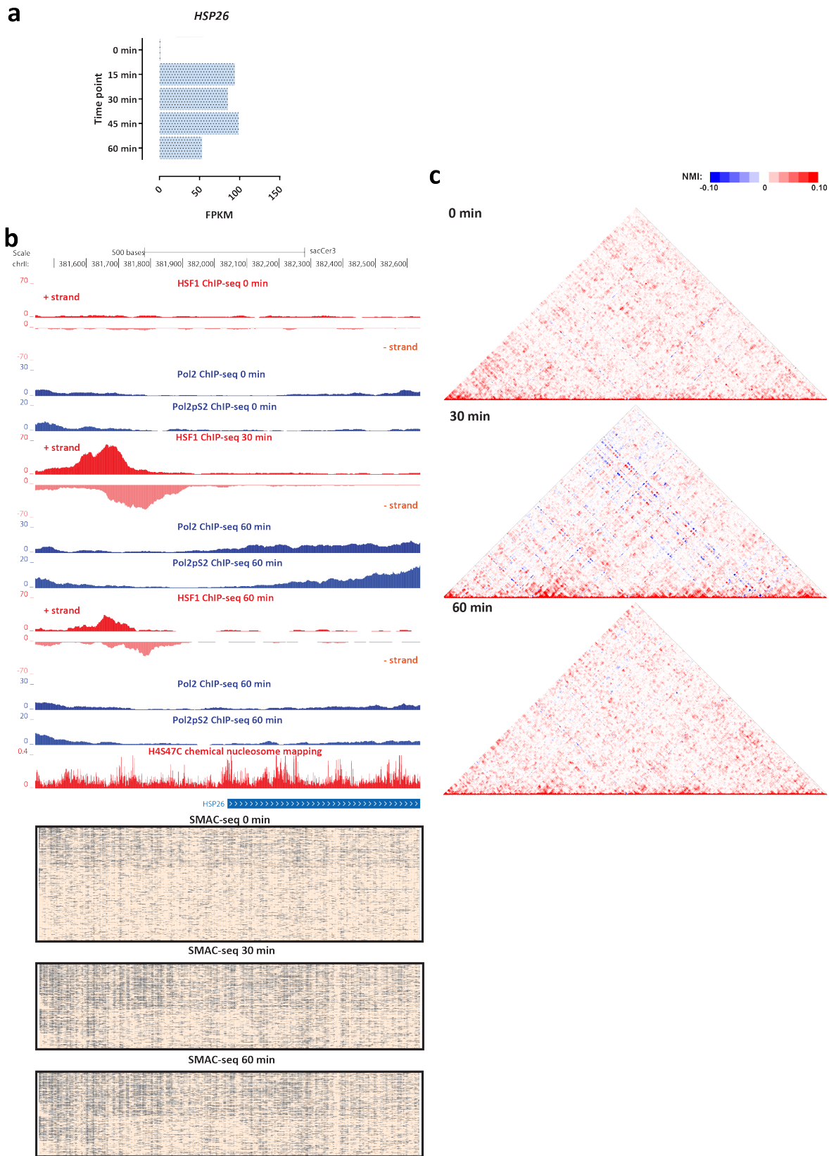
Supplementary Figure 65: Coordinated changes in chromatin accessibility and nucleosomal occupancy during the yeast stress response. Shown are changes in RNA Polymerase and HSF1 occupancy (measured by ChIP-seq), SMAC-seq profiles (1-bp resolution, 10-bp aggregate scores) and NMI profiles in the vicinity of the HSP26 gene.
