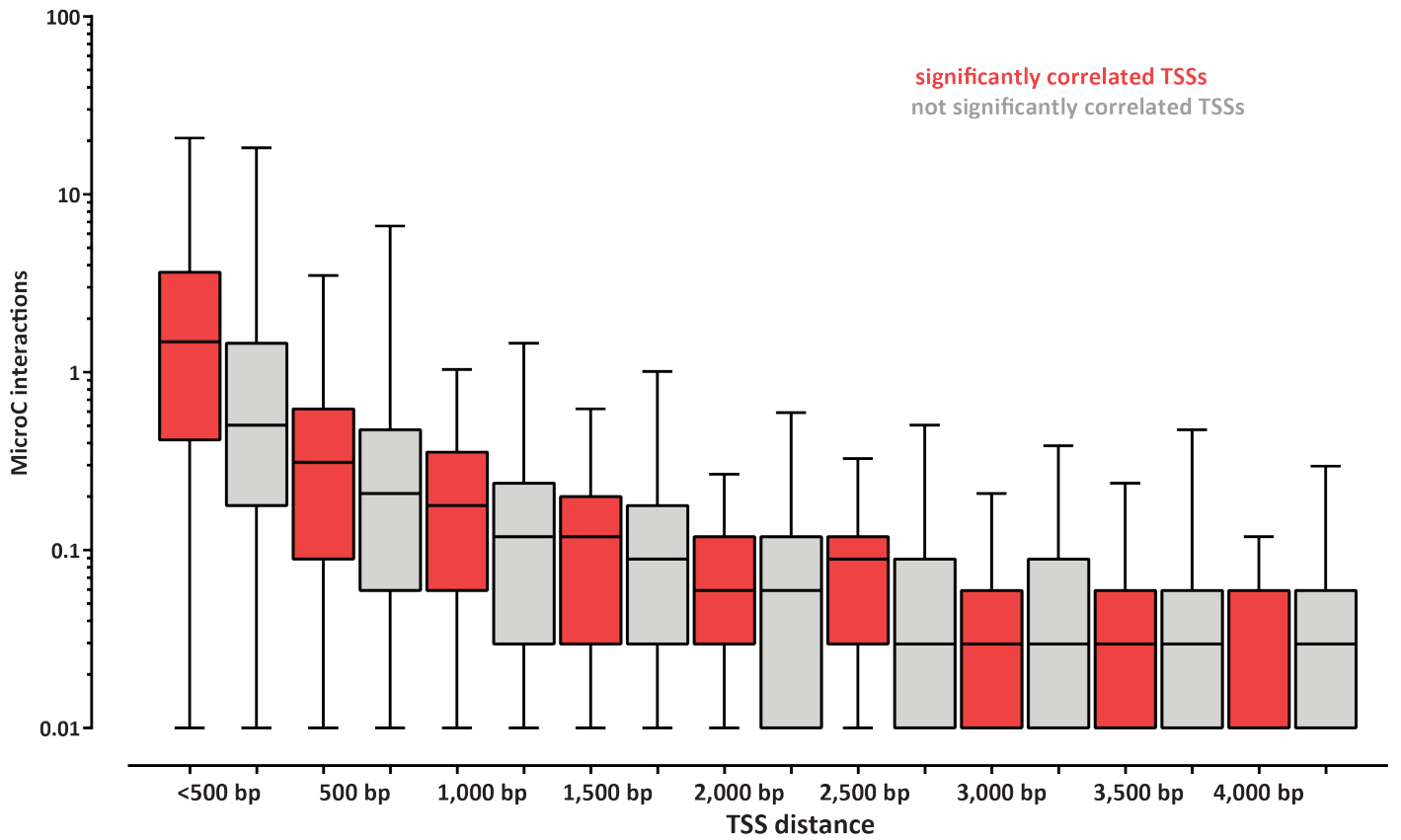
Supplementary Figure 59: Accessibility correlation between TSSs and 3D interactions. Shown are significantly and non-significantly correlated TSSs (defined as the regions \pm 100 bp around the TSS) split into distance bins and the number of 3D interactions between each group (measured by MicroC).
