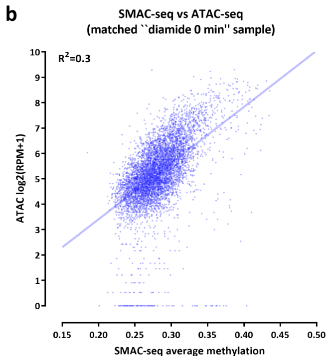
Supplementary Figure 23: Correlation of SMAC-seq signal with ATAC-seq and DNase-seq signal over yeast promoters. Shown is the average methylation over the TSS \pm 200 bp for SMAC-seq and RPM (Reads Per Million mapped reads) values for DNase-seq (a) and ATAC-seq (b). Note that the DNase-seq dataset is obtained from an external study while the SMAC-seq and ATAC-seq ones are from the same sample ("diamide 0 min repl").
