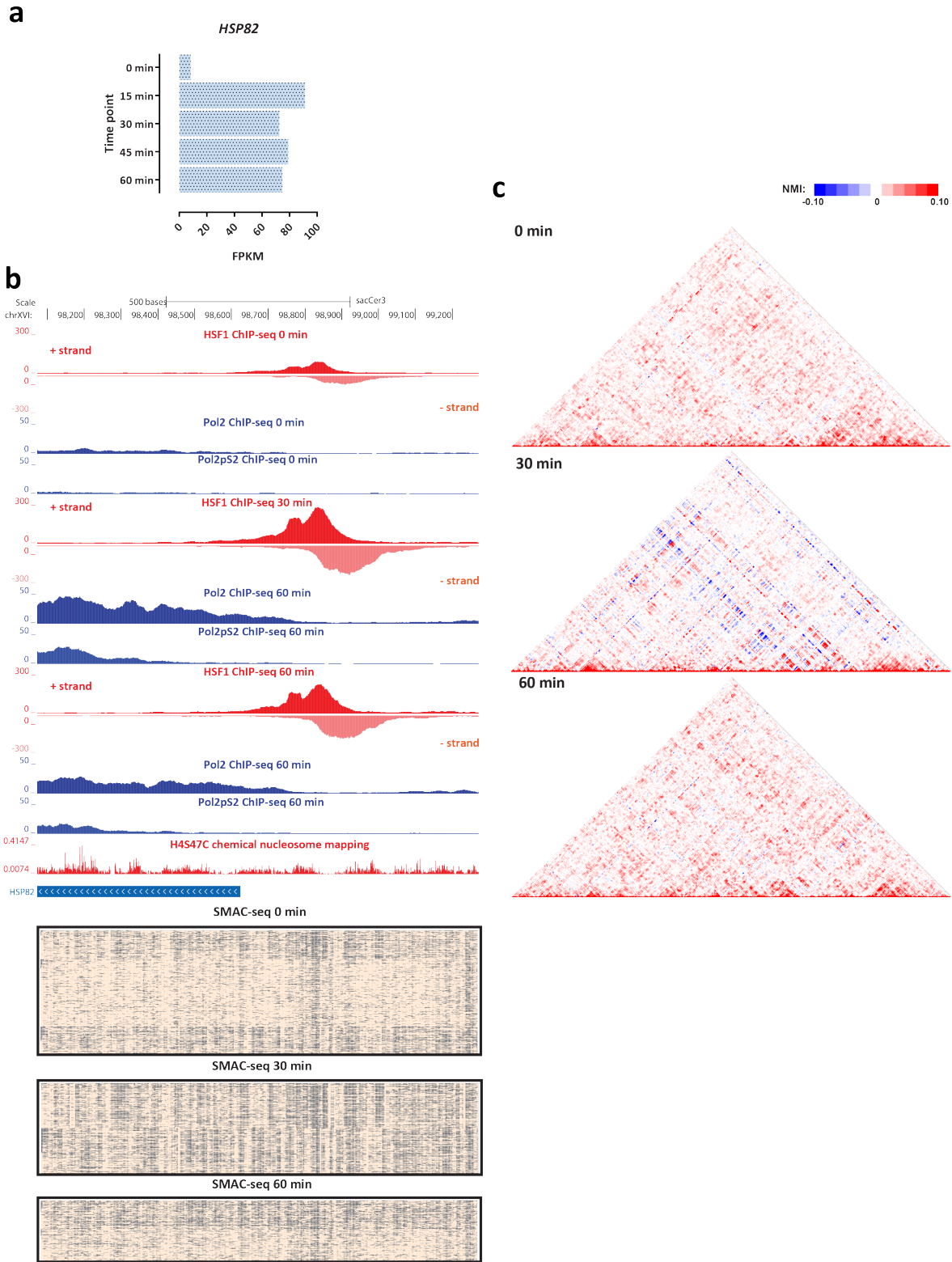
Supplementary Figure 68: Coordinated changes in chromatin accessibility and nucleosomal occupancy during the yeast stress response. Shown are changes in RNA Polymerase and HSF1 occupancy (measured by ChIP-seq), SMAC-seq profiles (1-bp resolution, 10-bp aggregate scores) and NMI profiles in the vicinity of the HSP82 gene.
