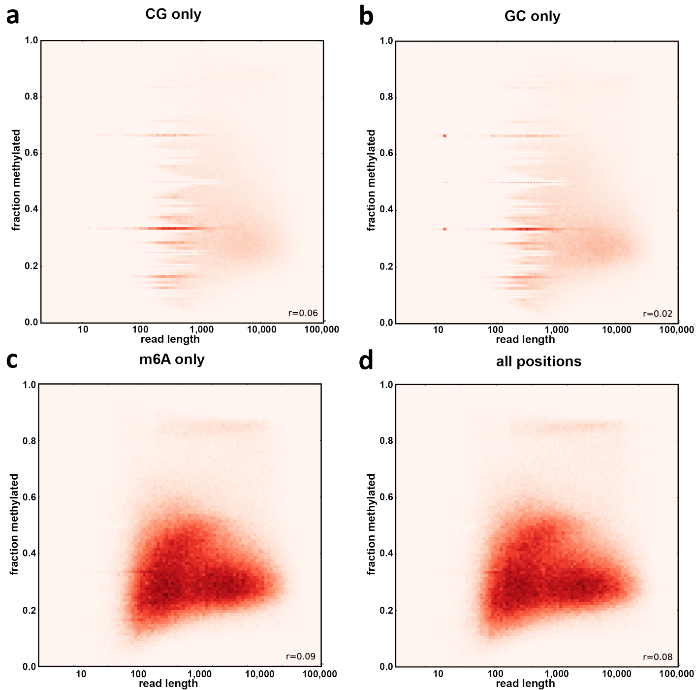
Supplementary Figure 17: Absence of strong correlation between nanopore sequencing read length and methylation status. Shown is the fraction of bases within each read that is scored as methylated. (a) CG positions only. (b) GC positions only. (c) m 6 A positions only. (d) All positions.
