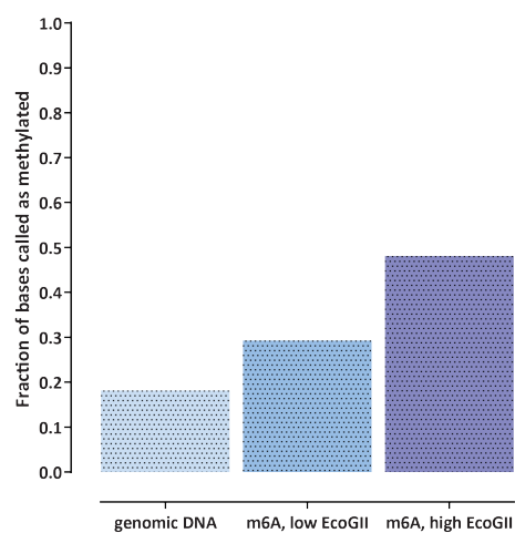
Supplementary Figure 5: Global m 6 A methylation levels in positive and negative controls (measured by nanopore sequencing). Genomic DNA was incubated with no or a low/high amount of the EcoGII enzyme and then subjected to nanopore sequencing. Shown are the average methylation levels for A nucleotides. Note that completely methylated DNA molecules are not sequenced well on the nanopore platform (See also Supplementary Table 1), thus the methylation estimates in the treated samples are most likely underestimates.
