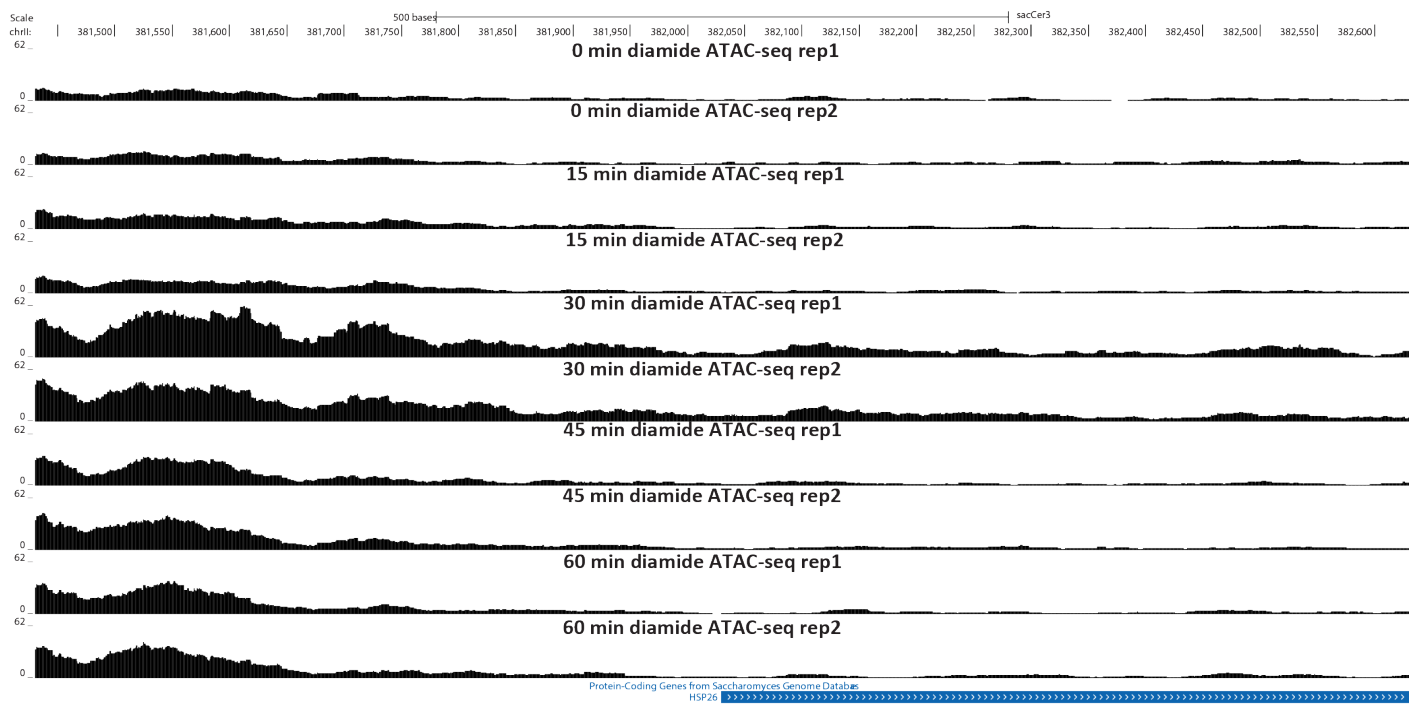
Supplementary Figure 77: Changes in chromatin accessibility during the yeast stress response around the HSP26 gene as measured by ATAC-seq.
