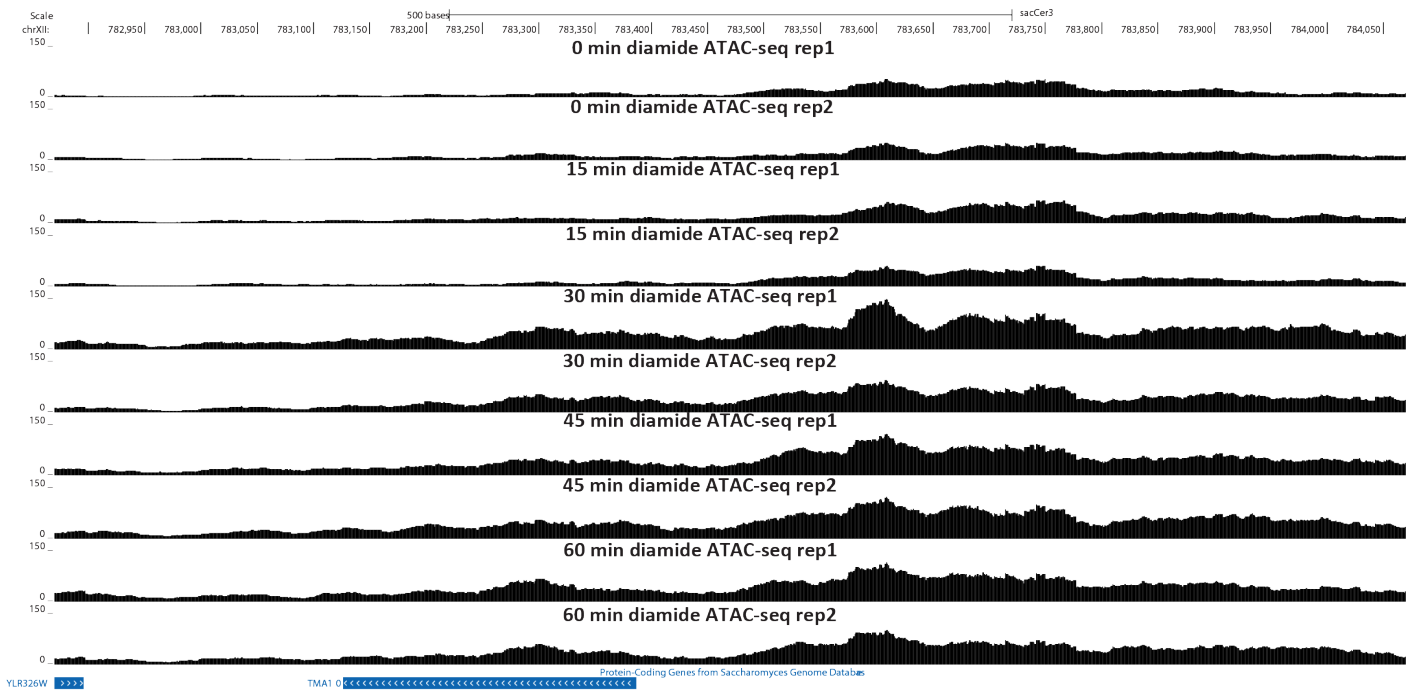
Supplementary Figure 76: Changes in chromatin accessibility during the yeast stress response around the TMA10 gene as measured by ATAC-seq.
