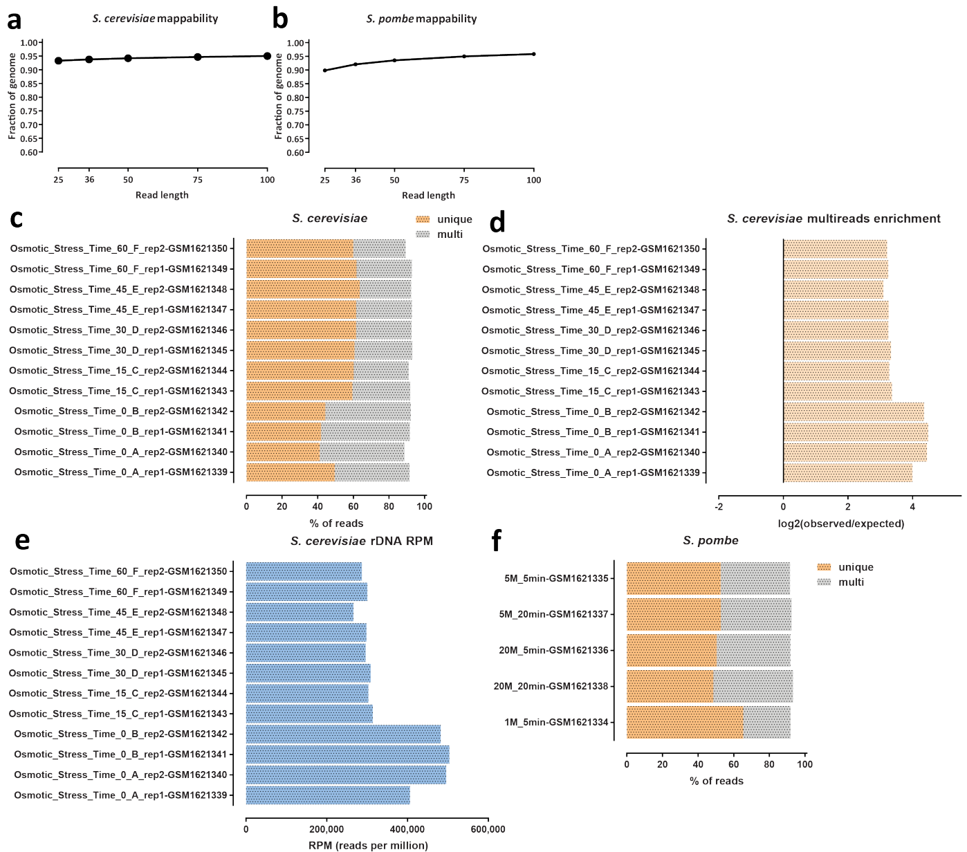
Supplementary Figure 38: Ribosomal DNA arrays are highly enriched for chromatin accessibility as measured by ATAC-seq. (a) Unique read mappability of the Saccharomyces cerevisiae genome as a function of read length (b) Unique read mappability of the Schizosaccharomyces pombe genome as a function of read length (c and d) Enrichment of multimapping reads in Saccharomyces cerevisiae ATAC-seq datasets (e) ATAC-seq multireads are highly enriched for rDNA-mapping reads (f) Enrichment of multimapping reads in Schizosaccharomyces pombe ATAC-seq datasets ATAC-seq datasets were obtained from Schep et al. 2015 52
