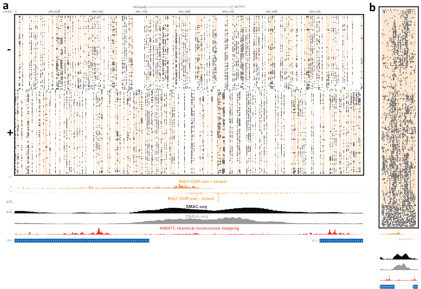
Supplementary Figure 44: Single-molecule footprinting by Reb1 binding sites. (a) Raw unfiltered nanopore reads fully spanning the 400-bp neighborhood of a Reb1 binding site on chrXVIII, at single-bp resolution. White spaces indicate positions for which there is no data (i.e. no CG, GC or A). (b) Same as in (a), but at aggregated 10-bp resolution.
