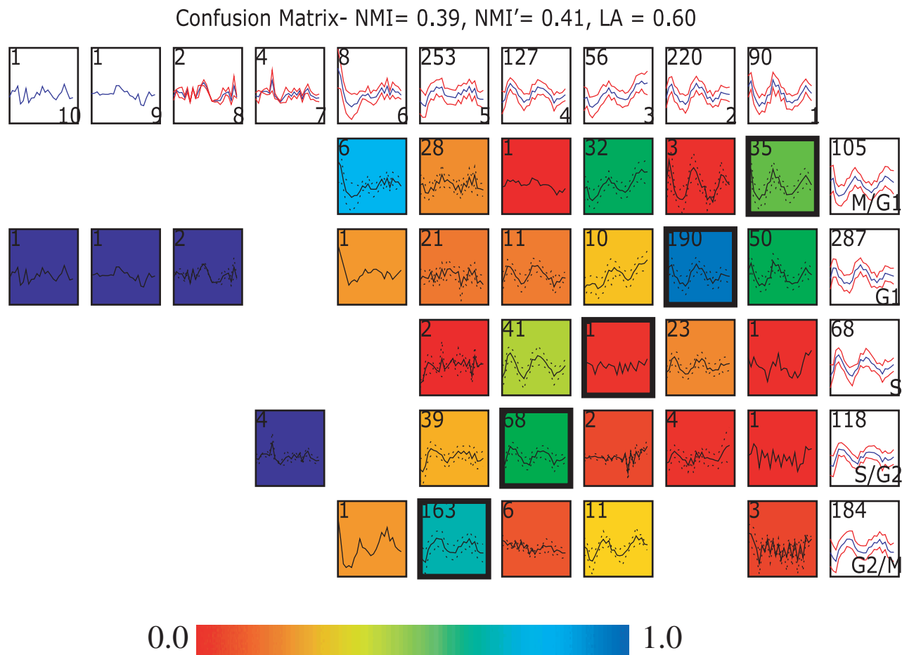
Figure 2. Comparing two clustering results on a ratiometric microarray dataset using a confusion array. Shown in this comparison is a Fourier clustering result published in the original study by Spellman et al. (16) and results from running an unsupervised clustering (Xclustagglom, see Methods) on the same ratiometric microarray dataset as the Fourier analysis was run on. Details of the figure layout are discussed in the legend of Figure 1. Here, the 5 Fourier clusters are shown along the rows, while the 10 Xclustagglom clusters are displayed across the columns.
