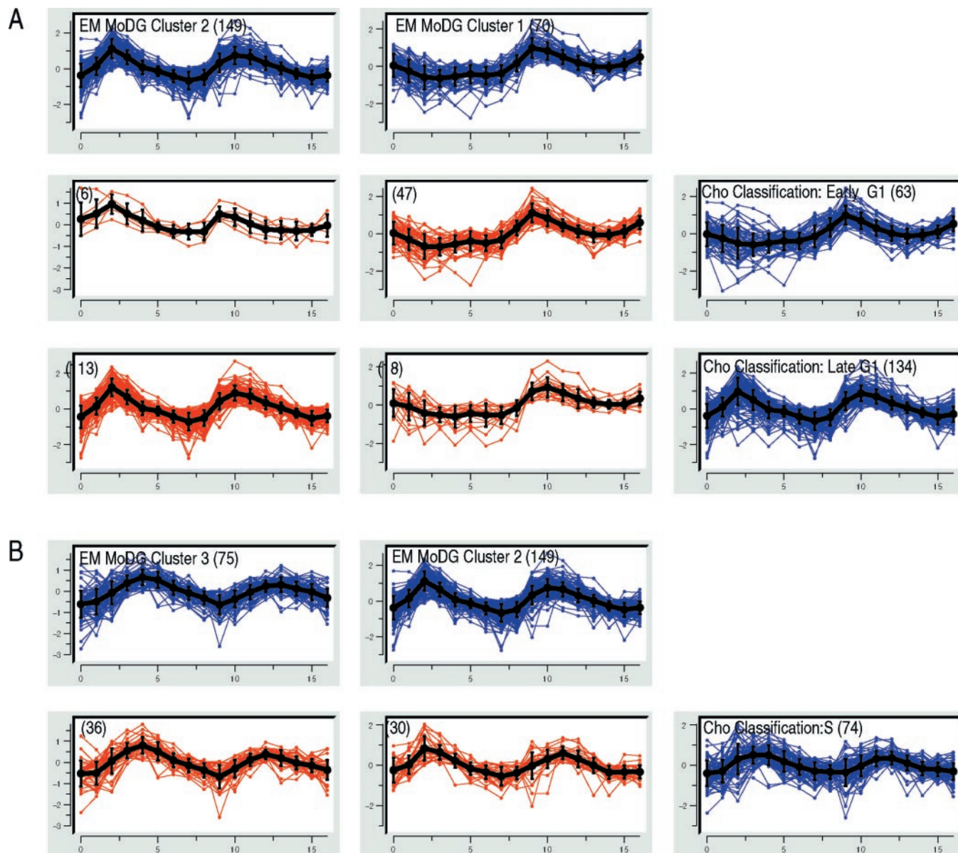
Figure 7. Selected confusion array cells from Figure 1 highlighting cluster membership differences for genes with peak expression during the G 1 and S phases of the cell cycle. The trajectory summaries display an expression profile for every gene with time along the x-axis and expression along the y-axis. Blue trajectory summaries show parent clustering results (EM MoDG along the columns, the Cho classification along the rows). Intersection cells from the confusion array are shown in red. Mean vectors for each gene set are shown in black with error bars proportional to the standard deviation. The total number of gene expression vectors in each cell is shown in parentheses. (A) G 1 genes are subdivided differently by the two algorithms. EM MoDG separates genes upregulated only during the second phase of the cell cycle from those upregulated during both the first and second cycles. The Cho classification separates G 1 based primarily on peak time in the second cycle. Figure 8 illustrates these observed kinetic distinctions being a result of these genes belonging to distinct regulatory modules. (B) Detailed comparison from the confusion array of Figure 1 showing the S-phase cluster of the Cho classification is subdivided nearly equally among EM2, EM3 (optimal match by LA) clusters.
