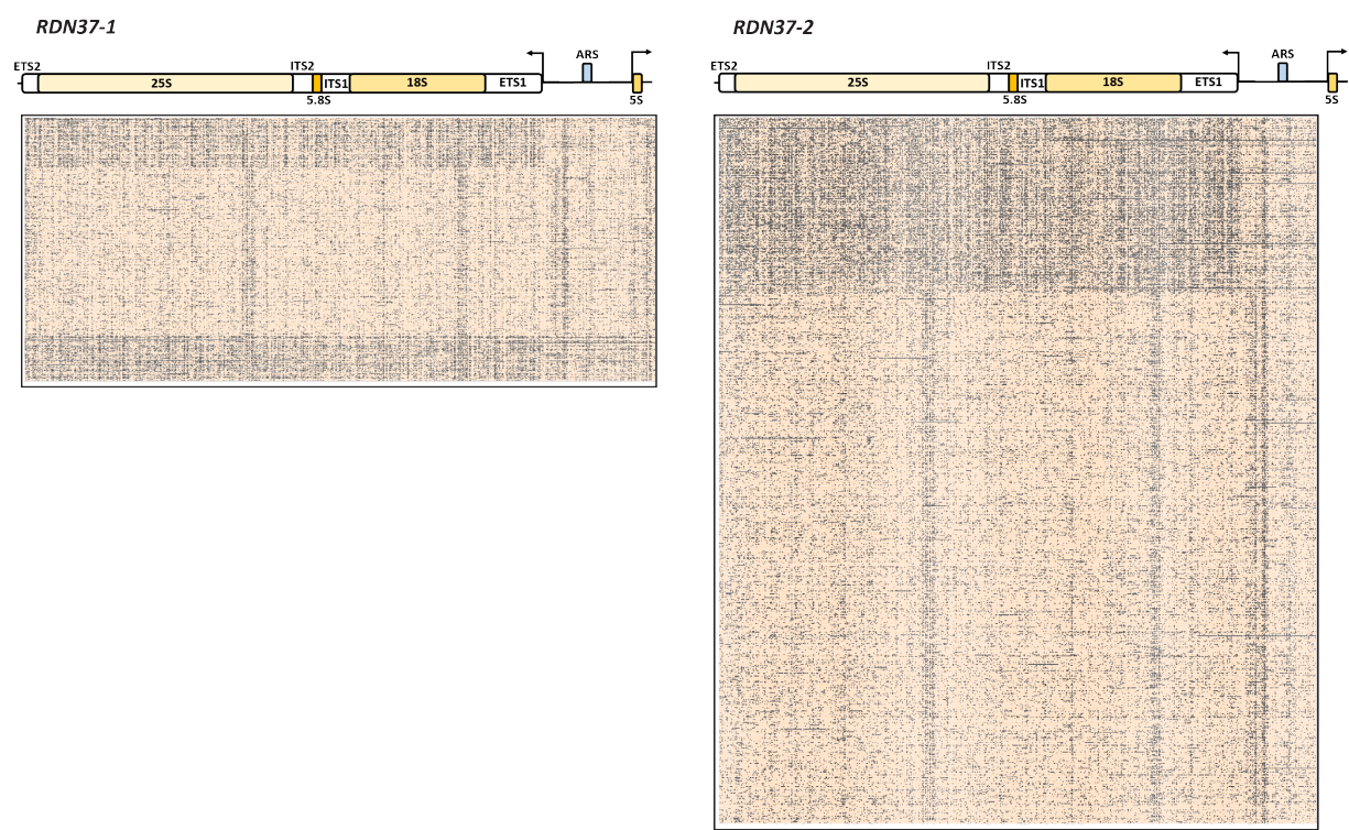
Supplementary Figure 39: SMAC-seq reveals the distribution of alternative chromatin states of rDNA arrays. Shown are all reads covering the RDN37-1 and RDN37-2 arrays in the RDN1 locus in the “diamide 0 min rep1” experiment (unfiltered reads, “aggregate” signal).
