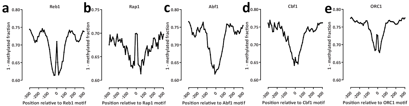
Supplementary Figure 42: Single-molecule footprinting by transcription factors. Shown is the average methylation status (averaged over 10bp) in the neighborhood of occupied (as measured by ChIP-exo or ChIP-seq) recognition motifs for several S. cerevisiae DNA binding proteins: (a) Reb1; (b) Rap1; (c) Abf1; (d) Cbf1. (e) ORC1. Strong footprinting is observed for Reb1, Rap1, and ORC1, while Abf1 and Cbf1 occupancy does not appear to be strongly protective against methylation.
