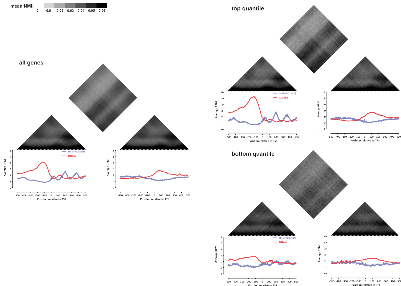
Supplementary Figure 53: Patterns of coaccessibility between the 5' and 3' ends of genes. Shown is the average NMI for the \pm 500\text{bp} regions in the 5' and 3' end of all yeast genes as well as the top and bottom 20% expression-ranked genes (calculated over 10-bp windows). Only genes \geq 1000 bp in length are shown. Similar results are obtained using windows of size 20bp or 50bp (data not shown).
