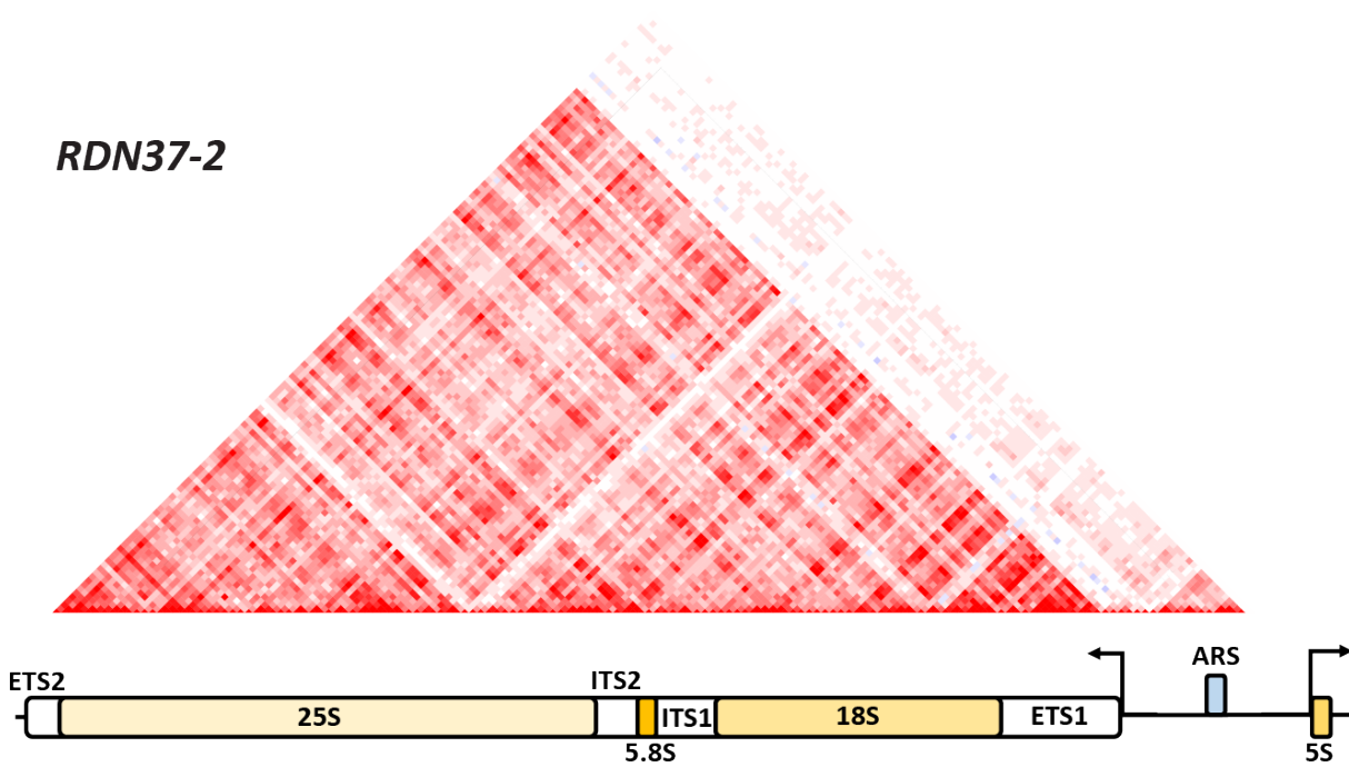
Supplementary Figure 40: NMI profile for the RDN37-2 array, as in Figure 3b.
