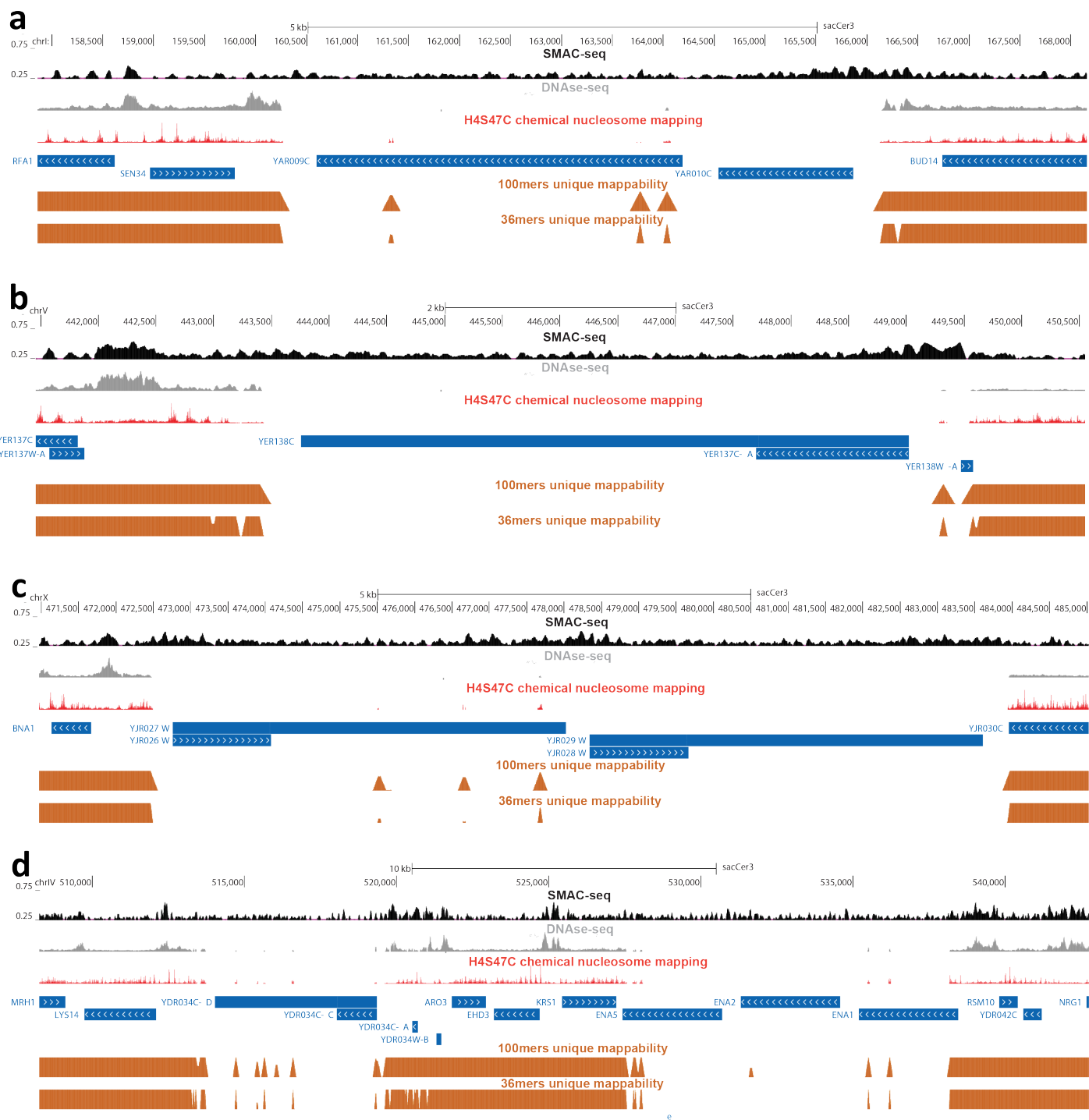
Supplementary Figure 31: SMAC-seq provides coverage of areas of the genome that cannot be uniquely mapped using short reads. Four different repetitive regions are shown (a, b, c and d) together with short read coverage for DNase-seq and chemical nucleosome mapping data and unique mappability tracks for 36mers and 100mers.
