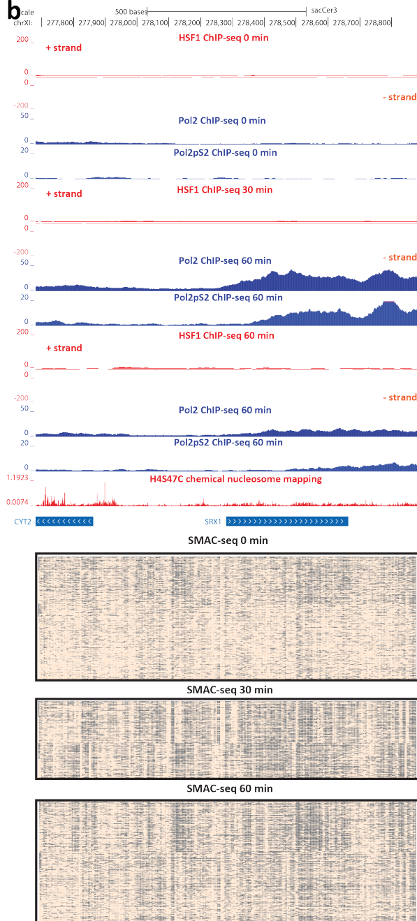
Supplementary Figure 66: Coordinated changes in chromatin accessibility and nucleosomal occupancy during the yeast stress response. Shown are changes in RNA Polymerase and HSF1 occupancy (measured by ChIP-seq), SMAC-seq profiles (1-bp resolution, 10-bp aggregate scores) and NMI profiles in the vicinity of the SRX1 gene.
