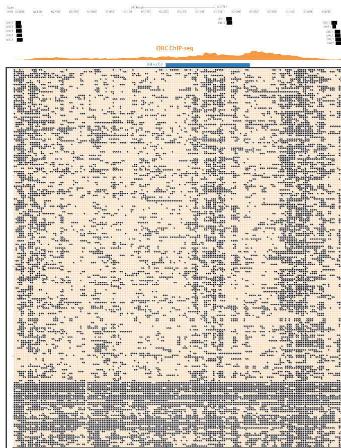
Supplementary Figure 50: Single-molecule footprinting associated with ORC occupancy. (a) Raw unfiltered nanopore reads fully spanning the neighborhood of an ARS site on chrII, at 5-bp aggregated resolution. White spaces indicate positions for which there is no data (i.e. no CG, GC or A).
