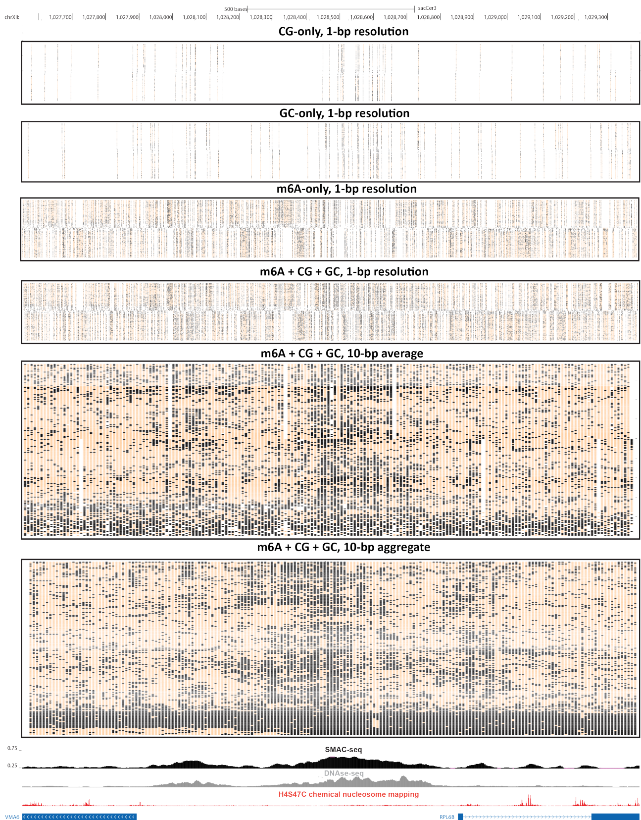
Supplementary Figure 4: Impact of the addition of m 6 A on assay resolution. Shown is the raw unfiltered nanopore read coverage around a divergent promoter region on chrXII, considering only CG, only GC, only m 6 A, and all bases at 1-bp resolution as well as all bases at averaged and aggregated 10-bp resolution. White spaces indicate positions for which there is no data (i.e. no CG, GC or A).
