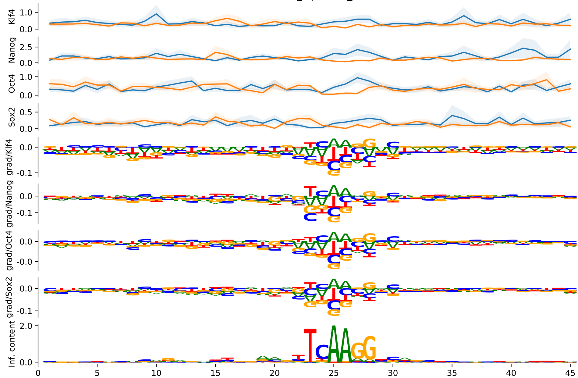
metacluster_6/pattern_6 (85)
