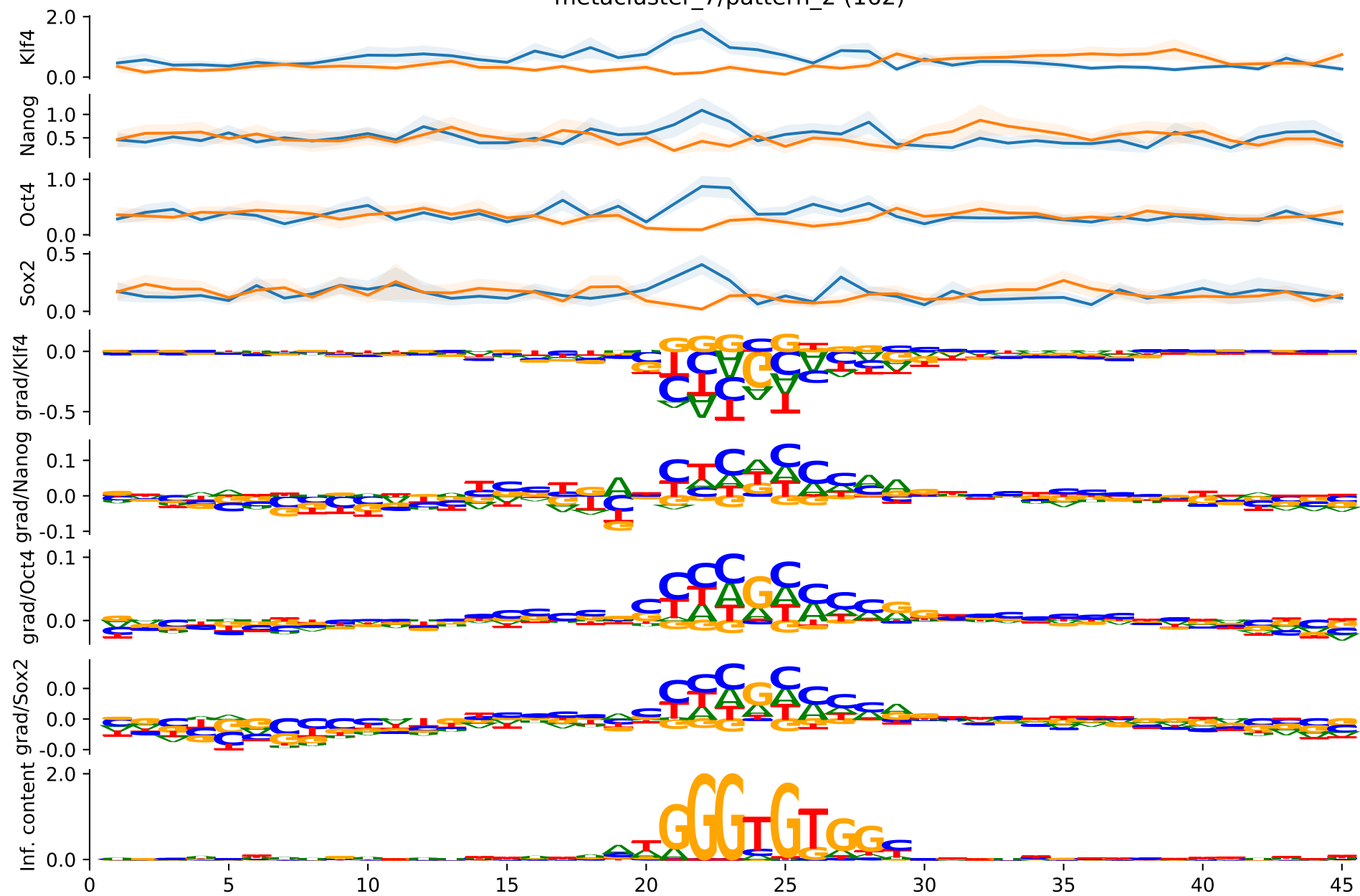
metacluster_7/pattern_2 (162)
