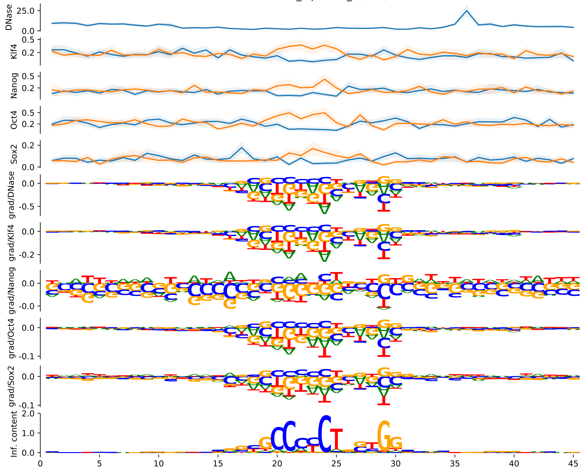
metacluster_8/pattern_0 (248)
