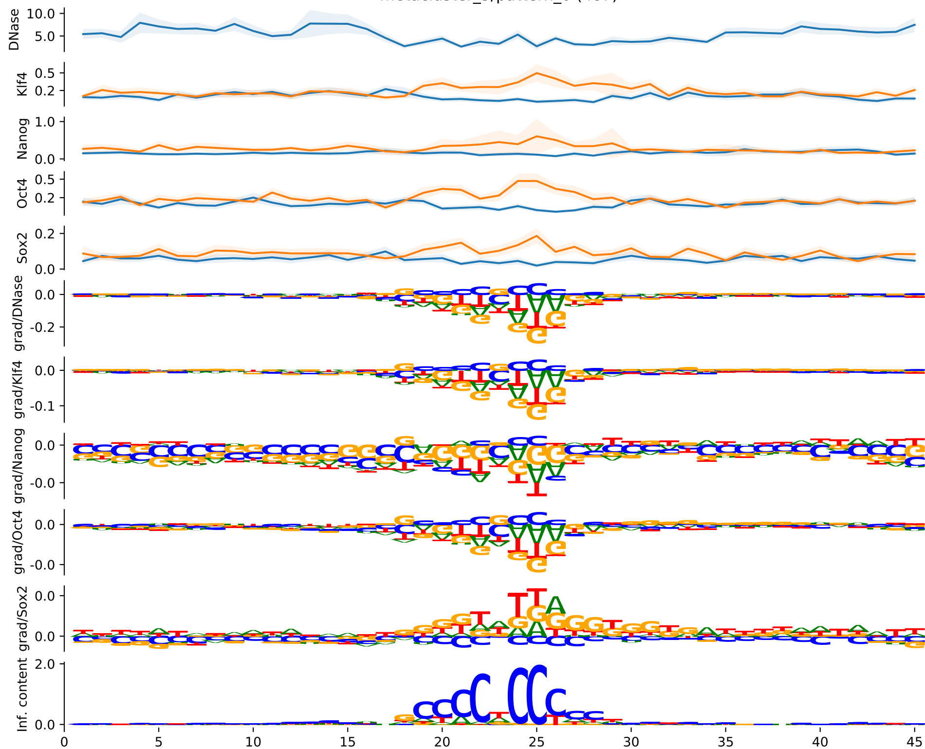
metacluster_5/pattern_0 (487)
