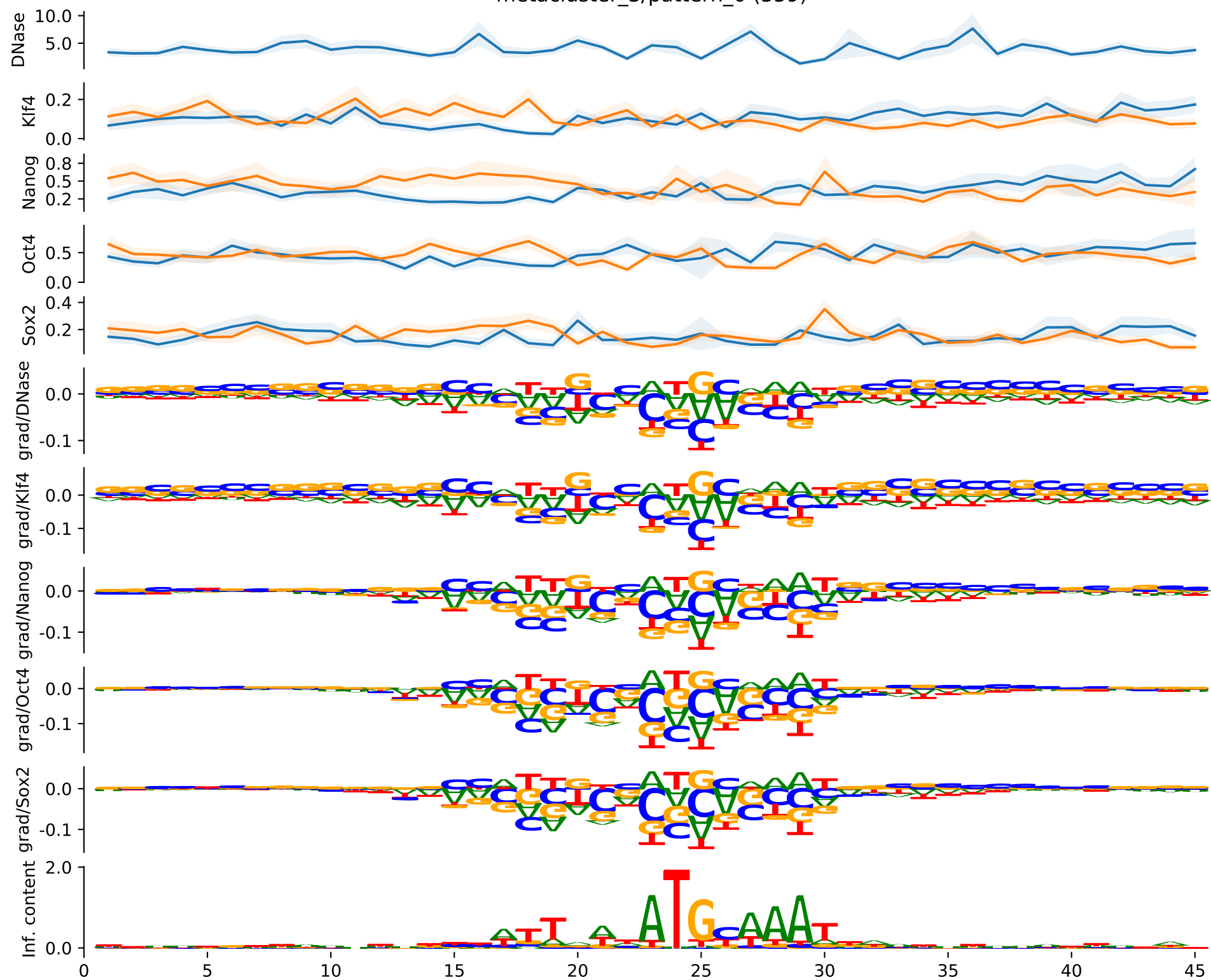
metacluster_3/pattern_0 (359)
