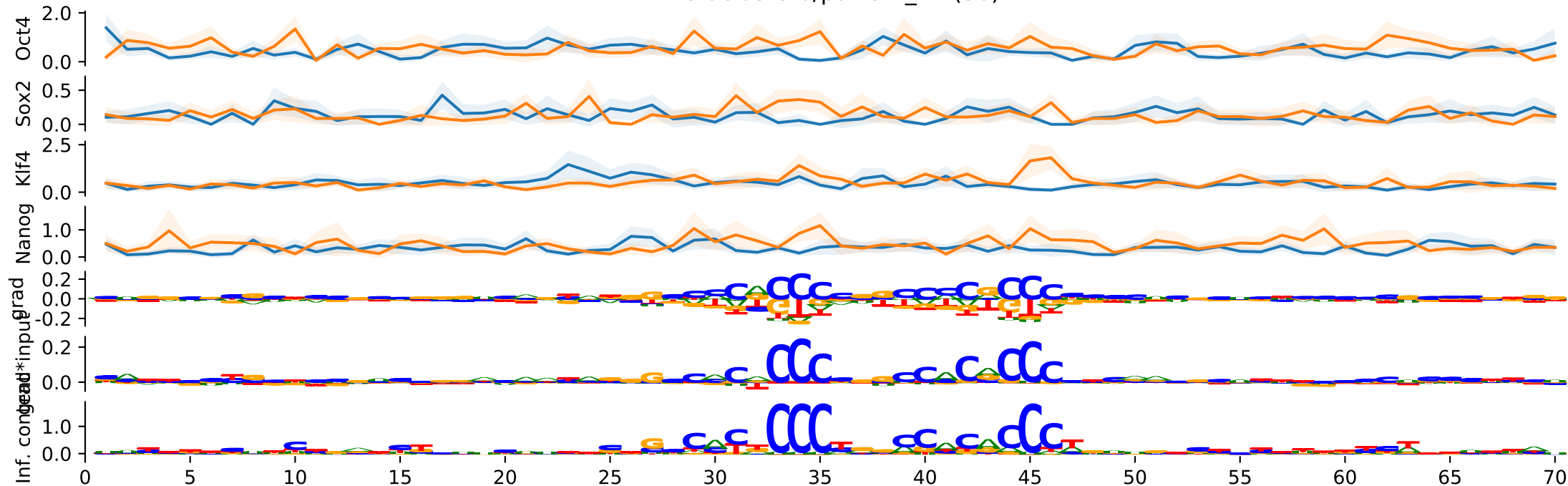
metacluster0/pattern_12 (36)
