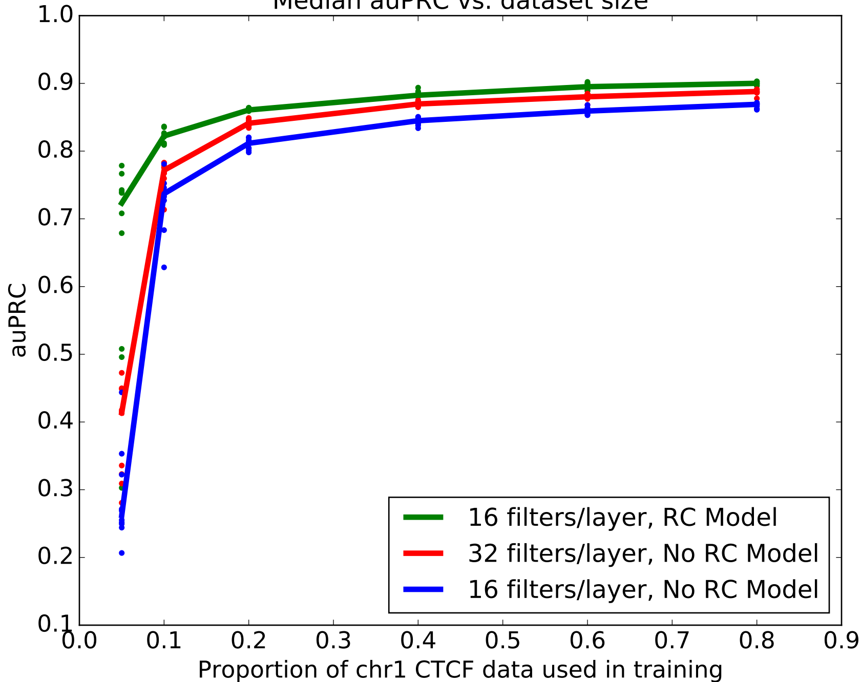
Median auPRC vs. dataset size
