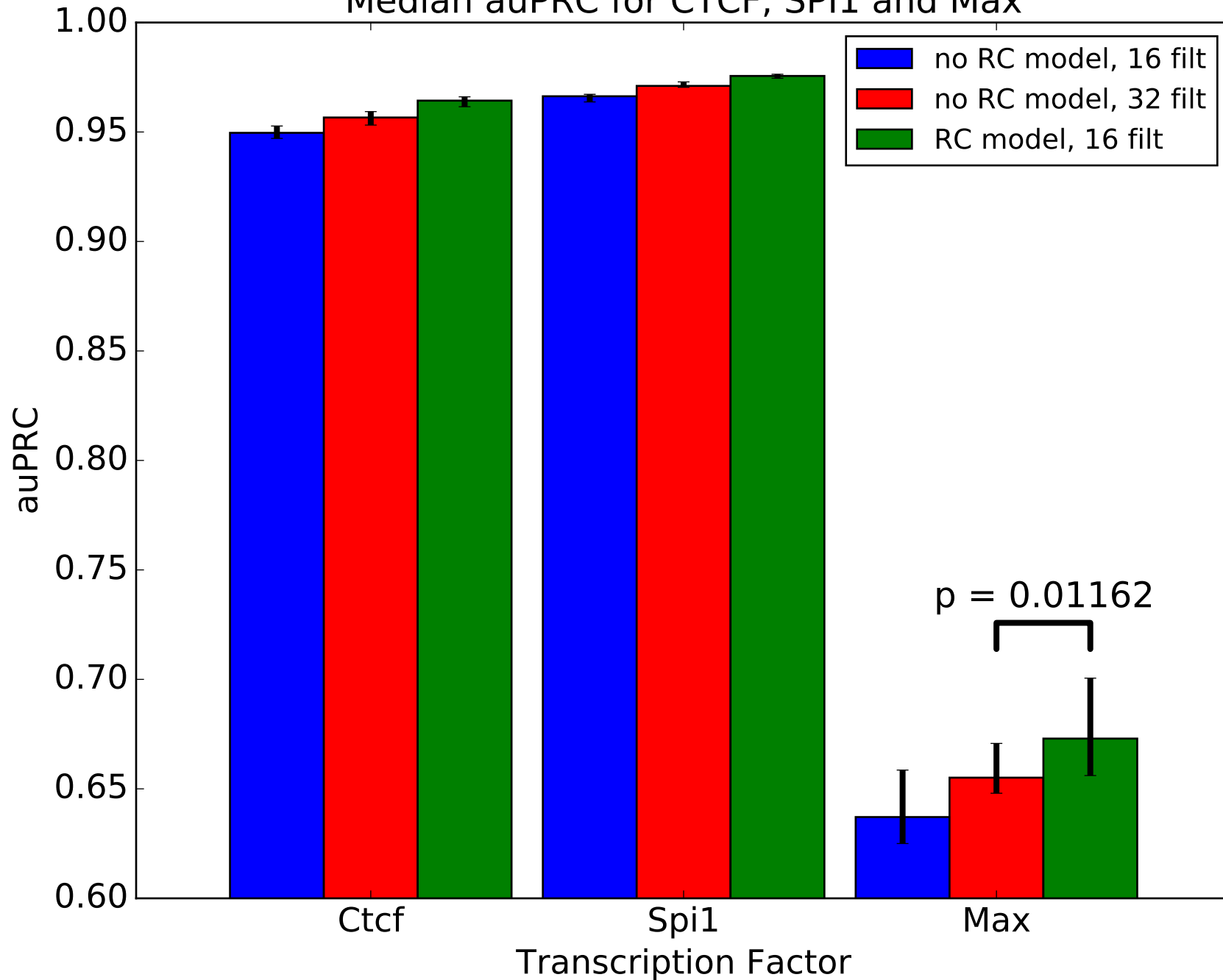
Median auPRC for CTCF, SPI1 and Max
