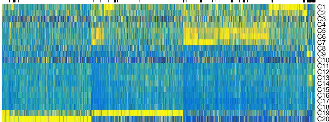
Column Z-Scores 3225 features GeneScoreMatrix -2 2
